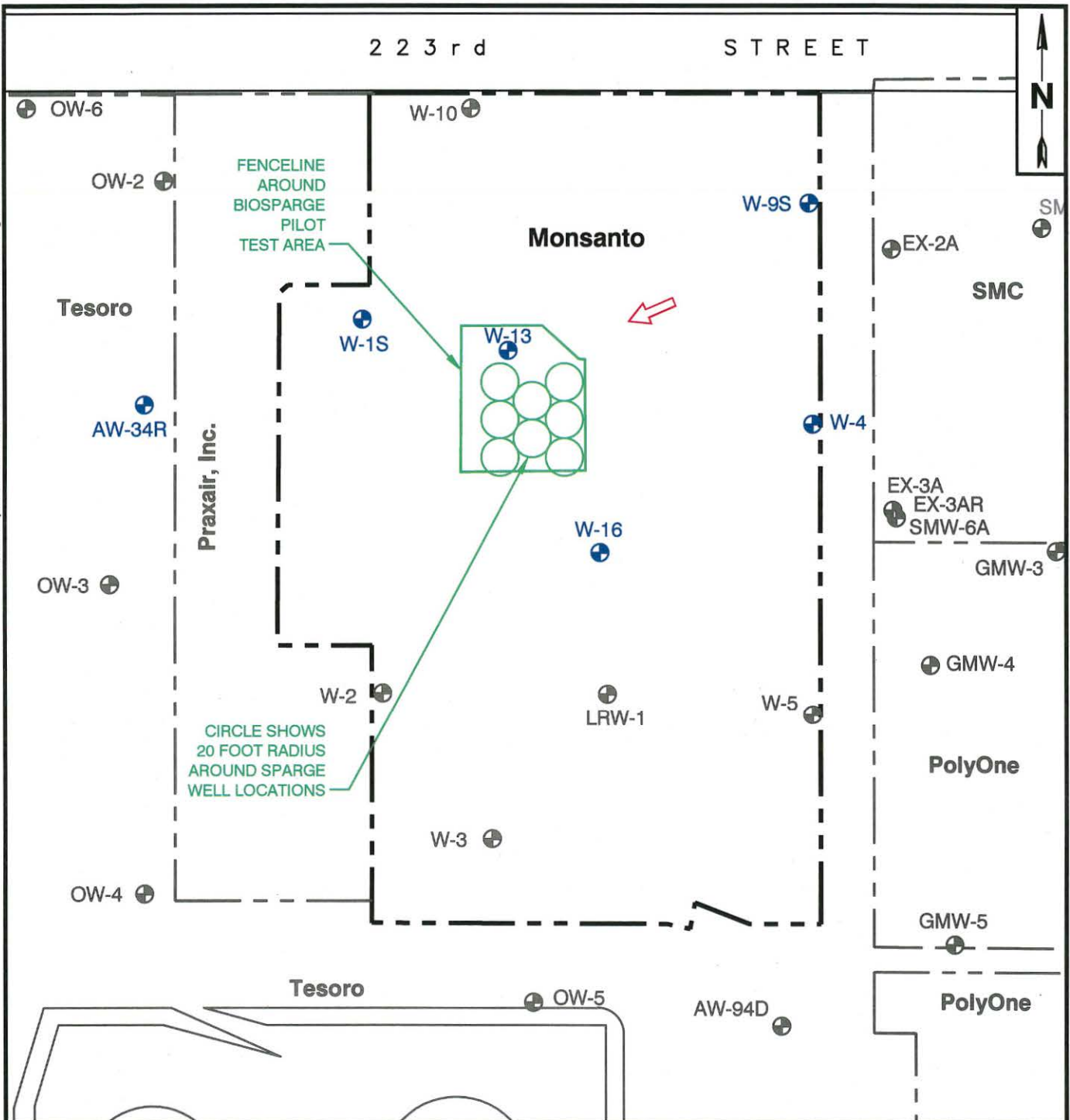
Figure 2 Site Plan Showing Biosparge Pilot Test Area and WDR Monitoring Wells
