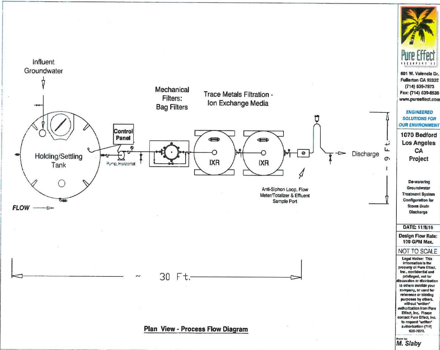
Figure 2. Treatment Schematic
