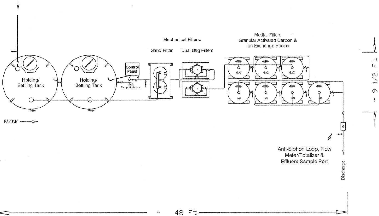
Figure 2. Treatment Process
