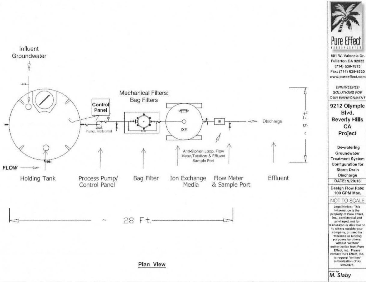
Figure 2. Treatment Flow Diagram
