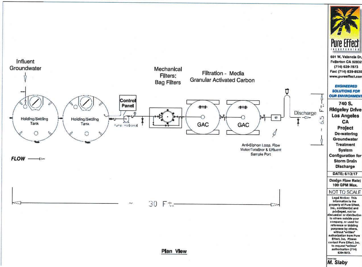
Figure 3. Treatment Flow Diagram
