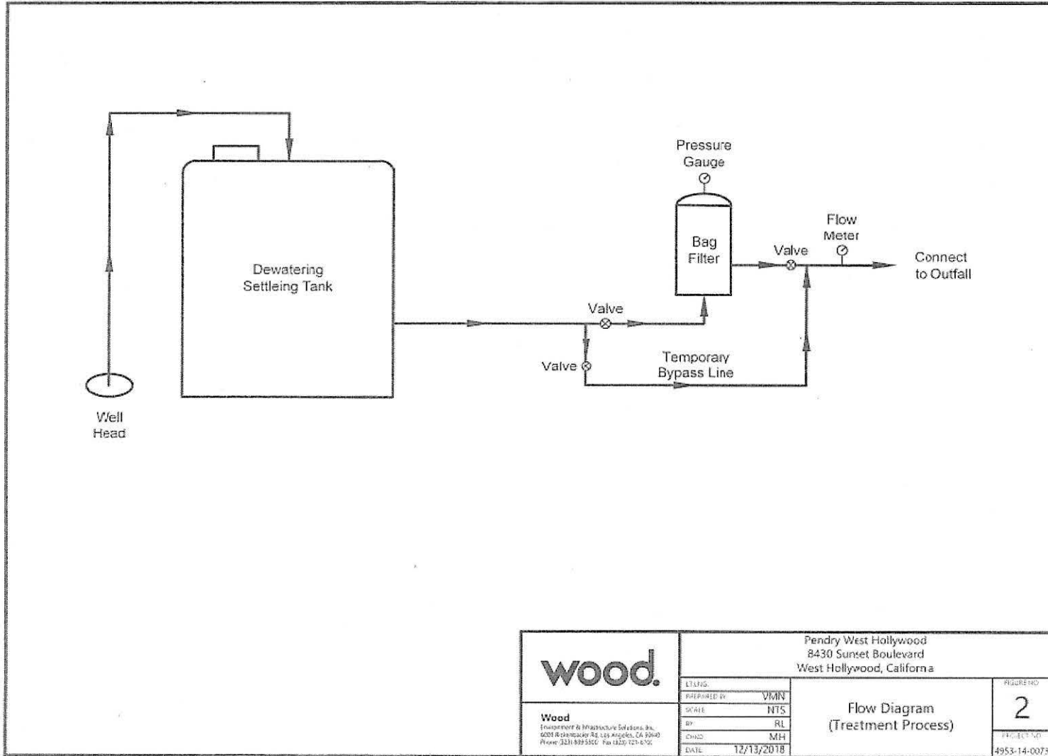
Fig Figure 2. Flow Schematic
