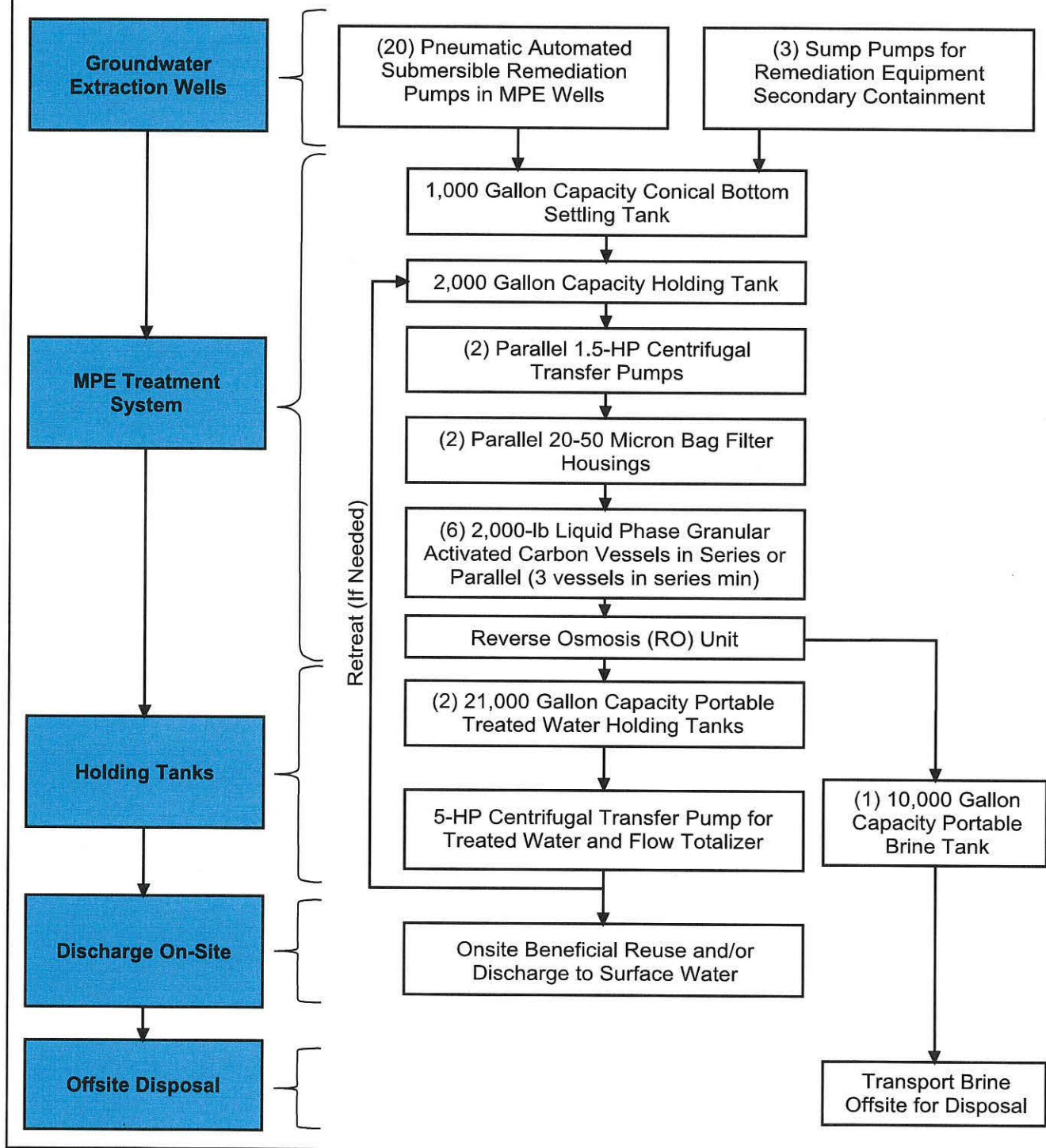
Figure 2. Treatment Process
