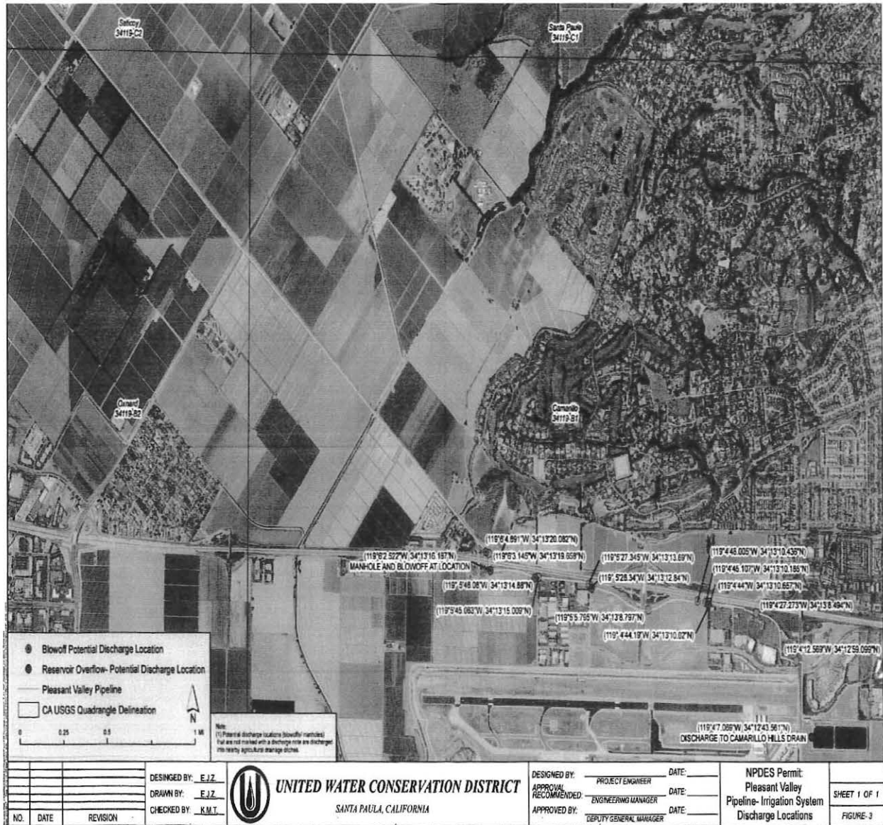
Figure 2. Site Map- Irrigation Water Distribution PV System Discharge Locations
