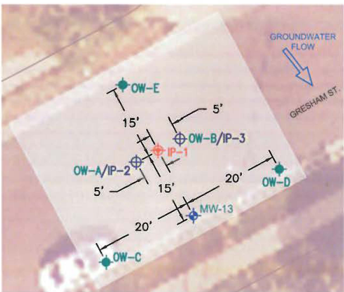
FIELD PILOT TEST STUDY AREA DETAIL (1" = 20')
