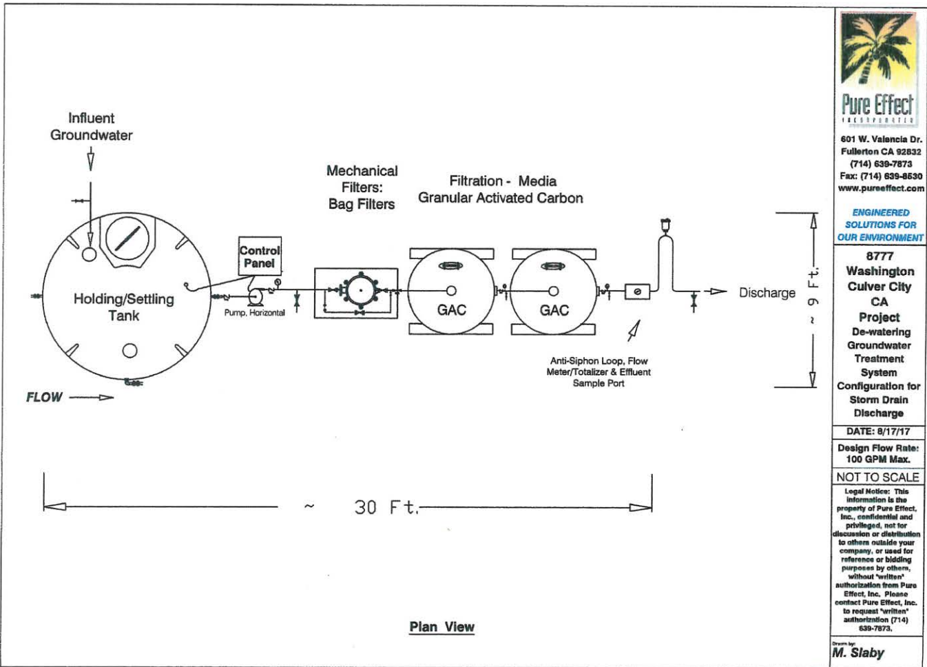
Figure 2. Treatment Schematic
