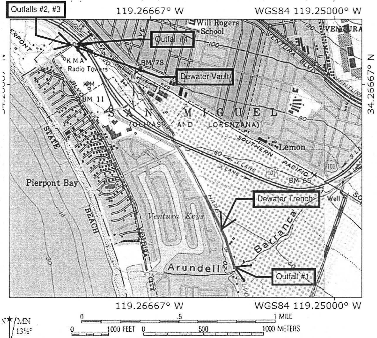
Figure 2. Outfall Locations Wastewater Main Force Project
