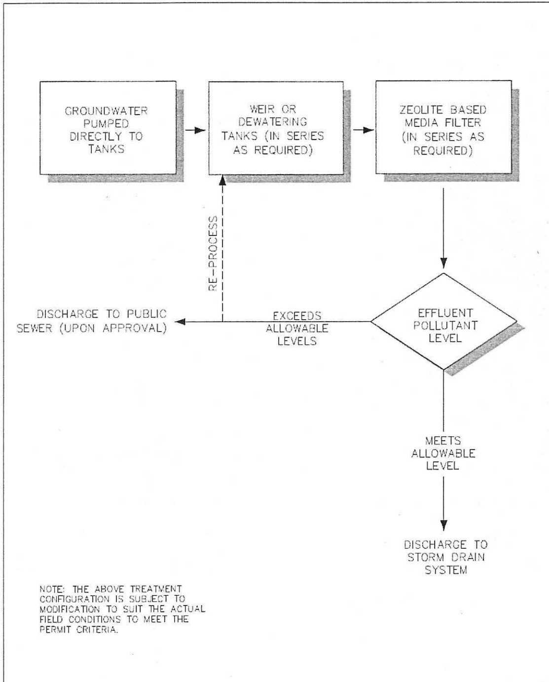
Figure 3. Treatment Flow Diagram
