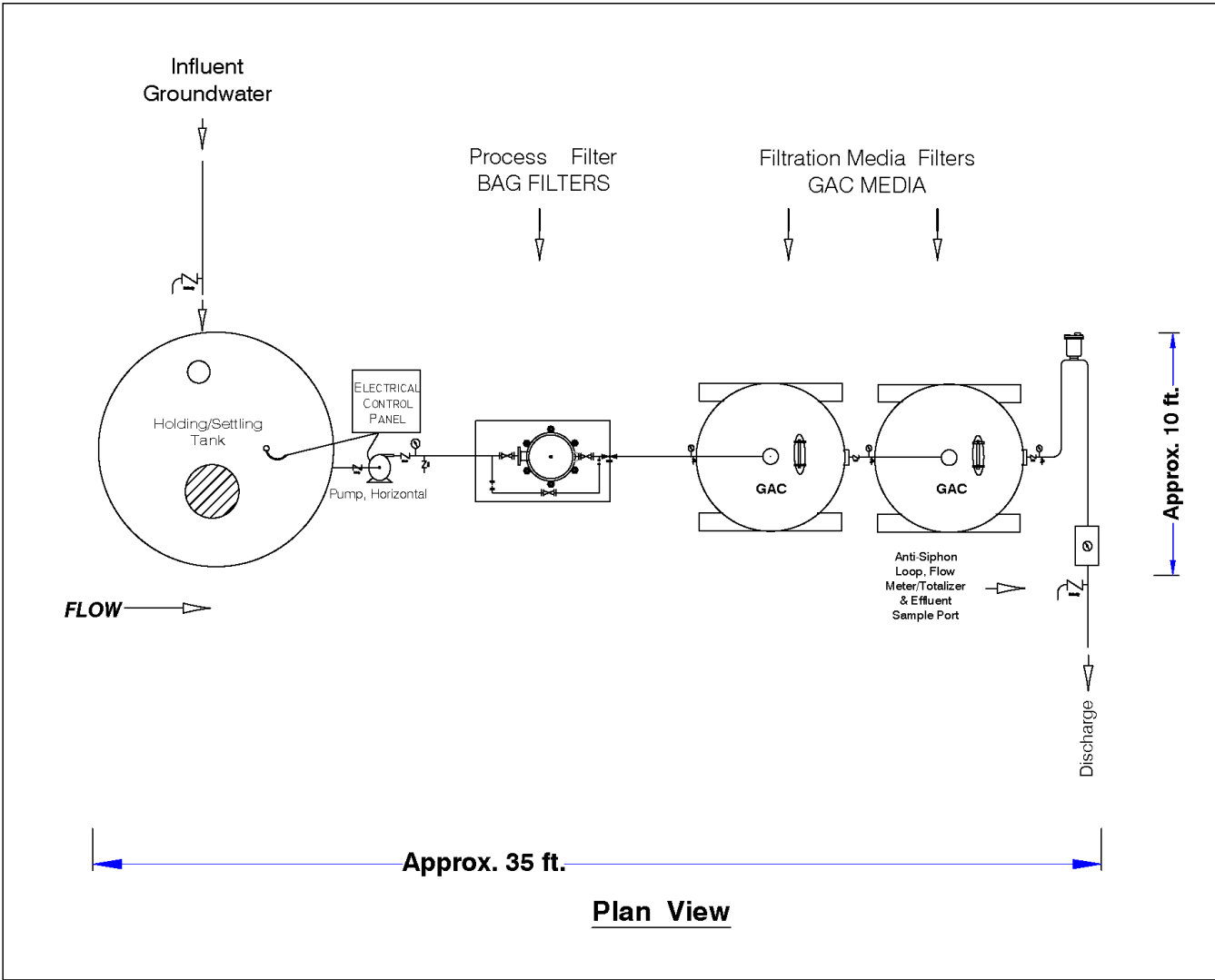
Figure 2. Treatment Process
