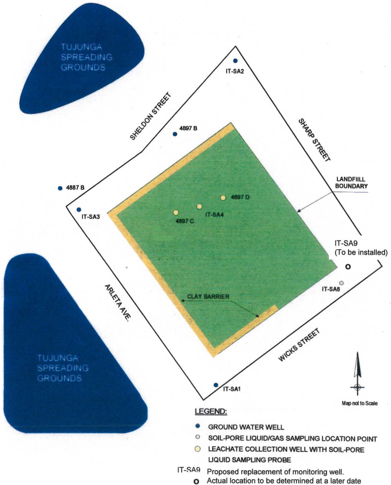
Figure 5. Existing Groundwater Well and Leachate Well Locations
