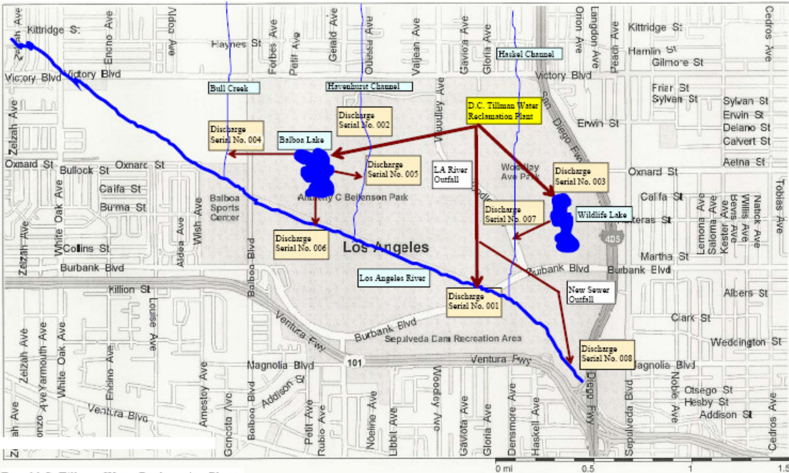
FIGURE 1 – The Vicinity Map and Water Quality Sampling Stations of the Donald C. Tillman Water Reclamation Plant
