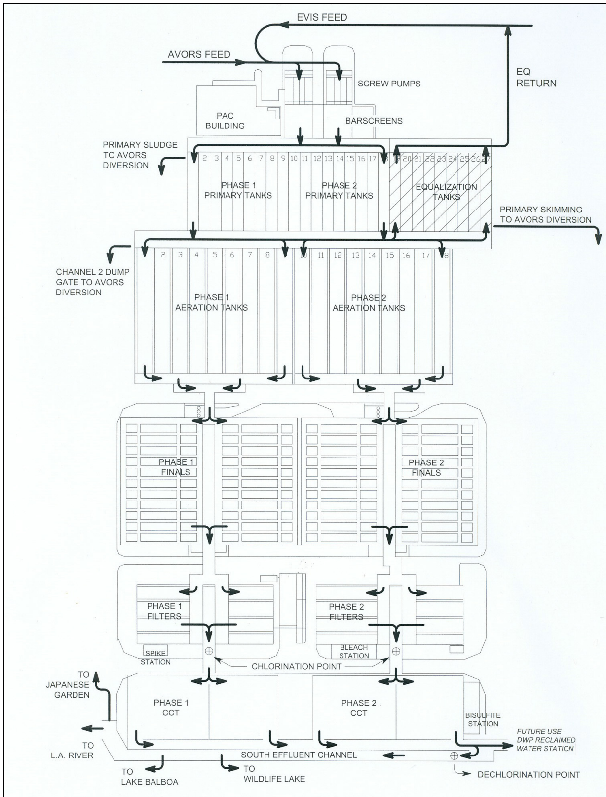
FIGURE 2 – The Flow Diagram of Wastewater Treatment Processes at the Donald C. Tillman Water Reclamation Plant
