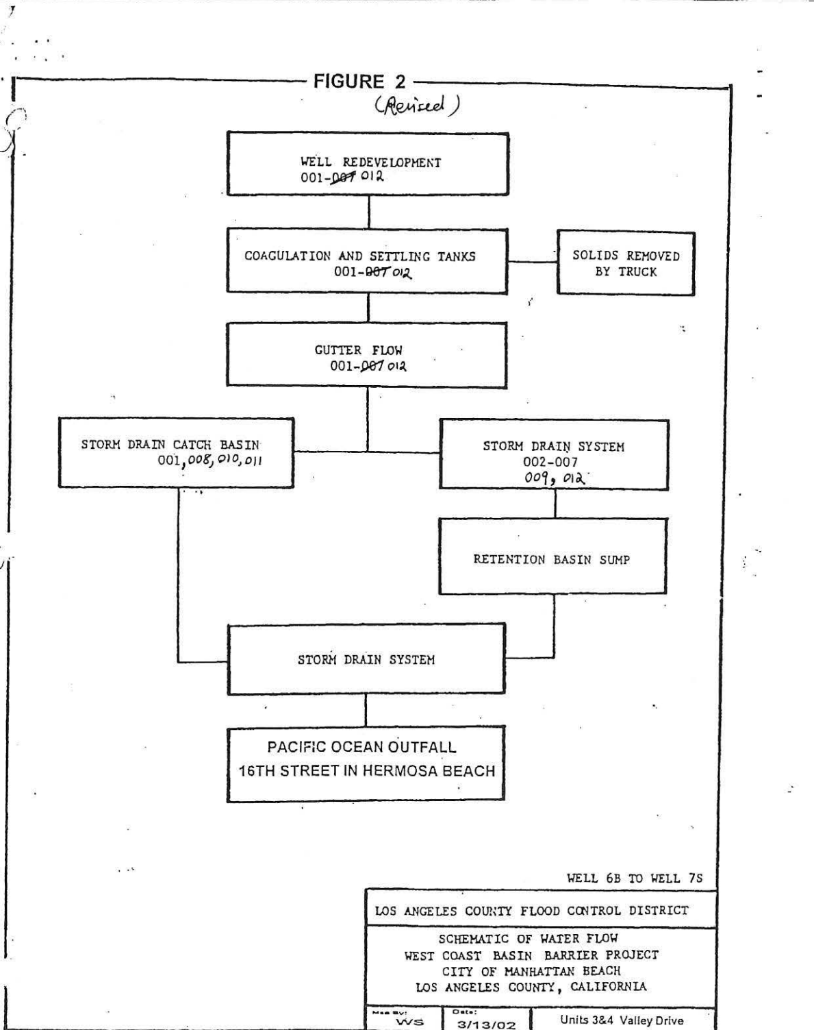
Figure 2. Schematic of Water Flow
