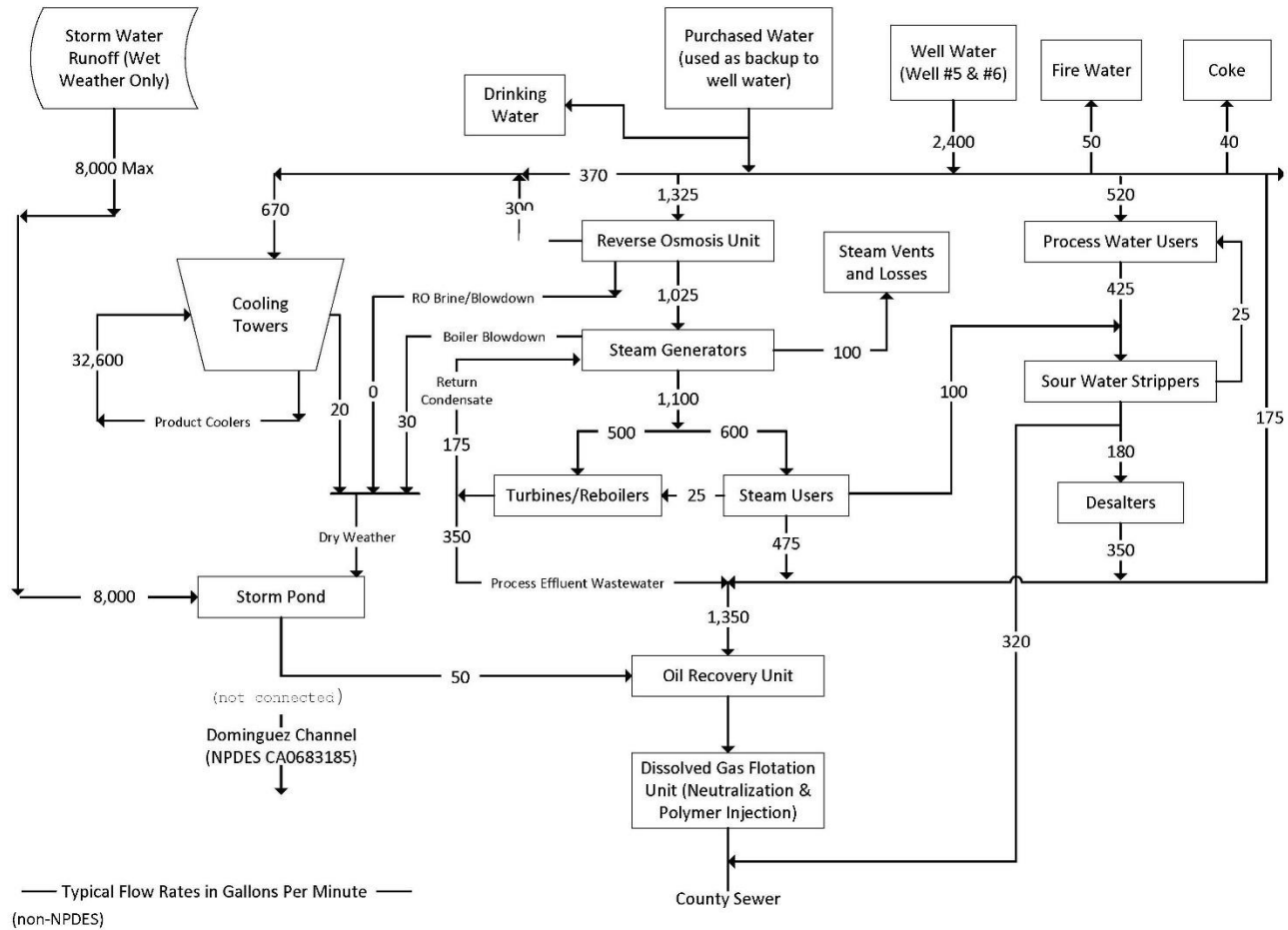
ATTACHMENT - FLOW SCHEMATIC STORM WATER FLOW MAP
