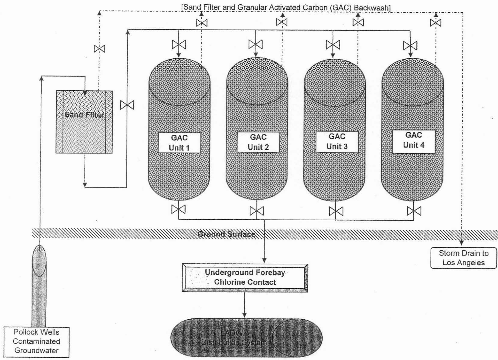
Figure 2 - Treatment Process
