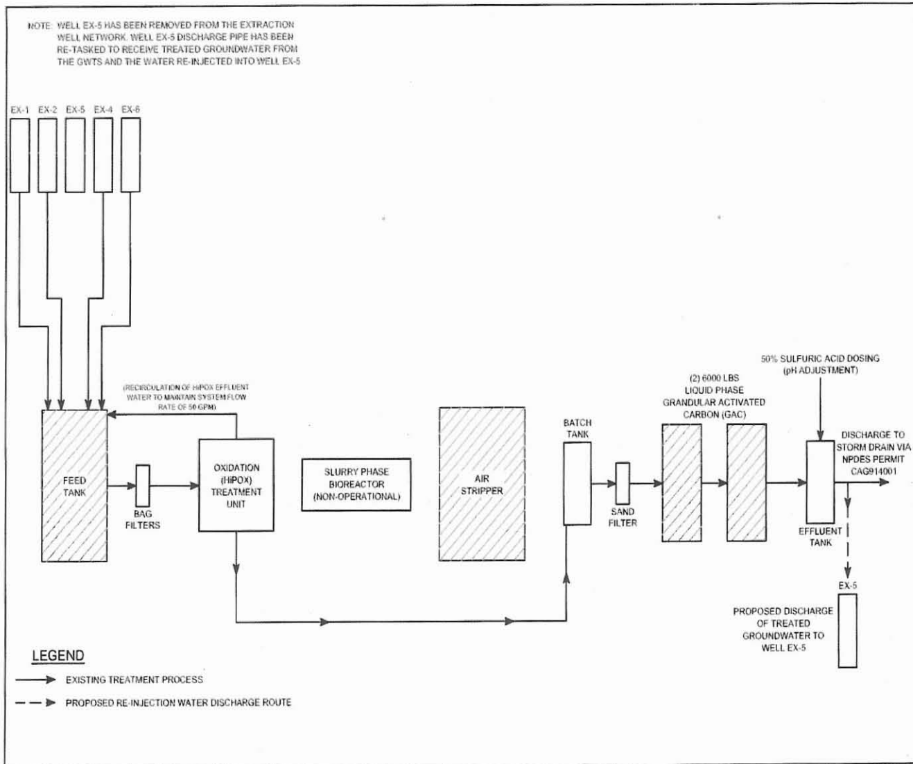
Treatment Schematic FIGURE 2
