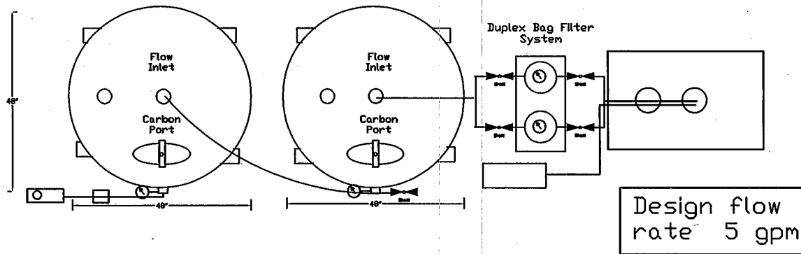
General Layout - Plan View
