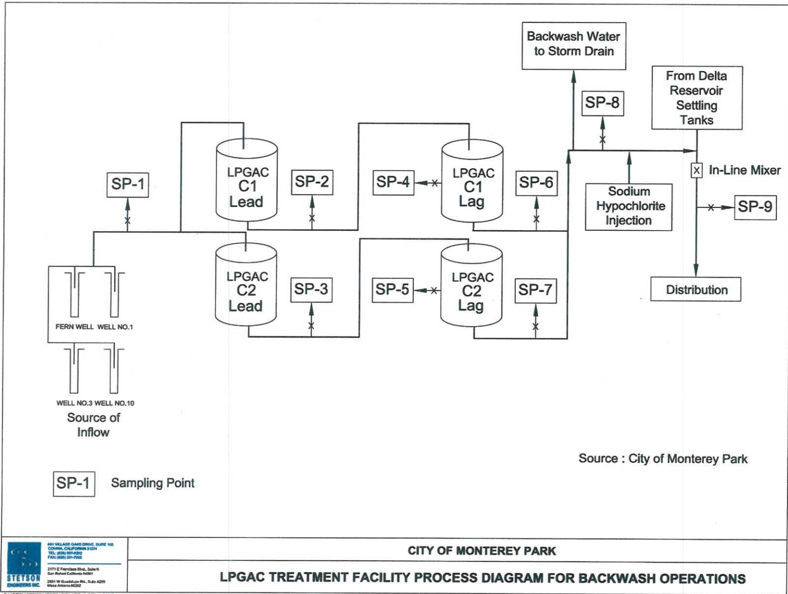
FIGURE 2-Treatment Facility No. 1
