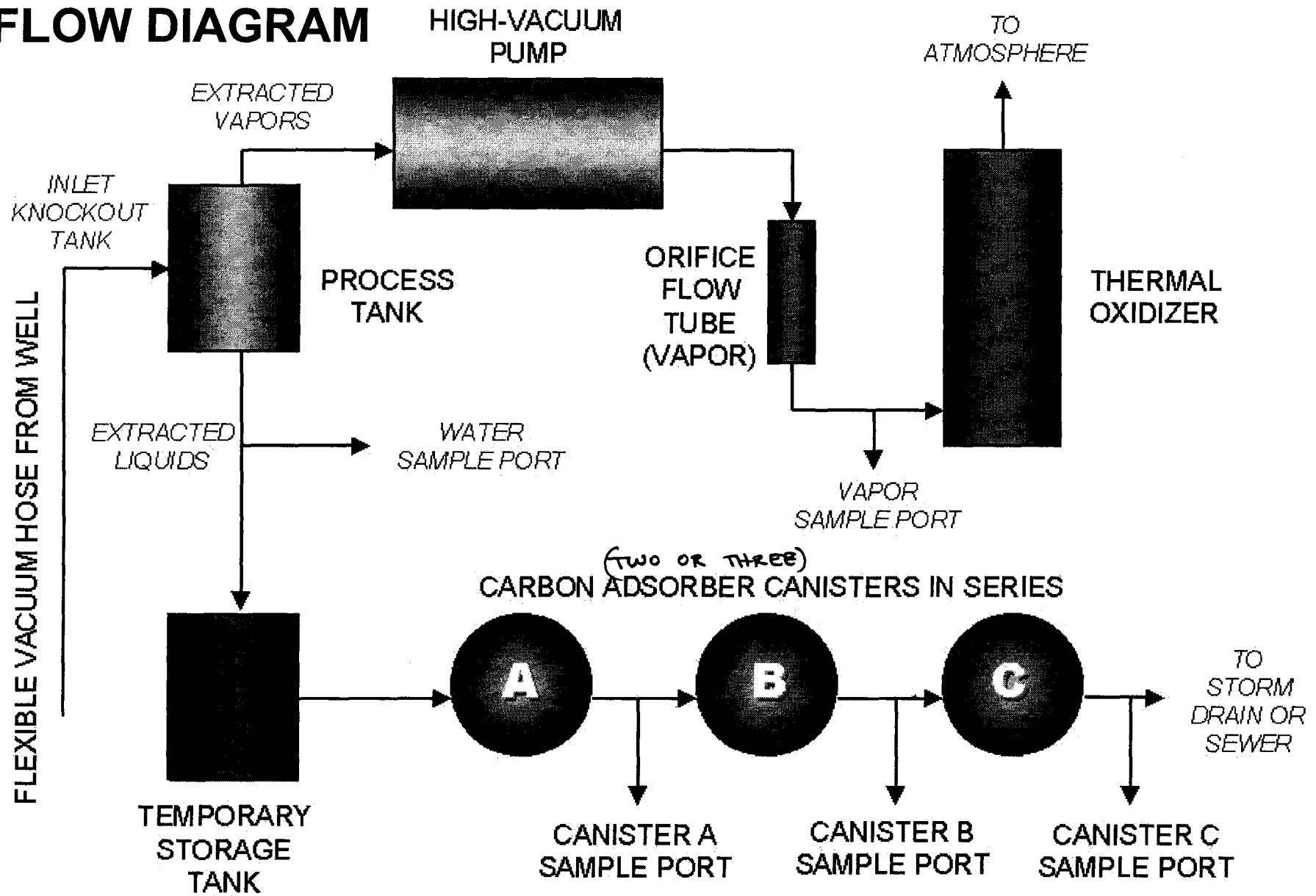
Figure 2. Treatment Process
