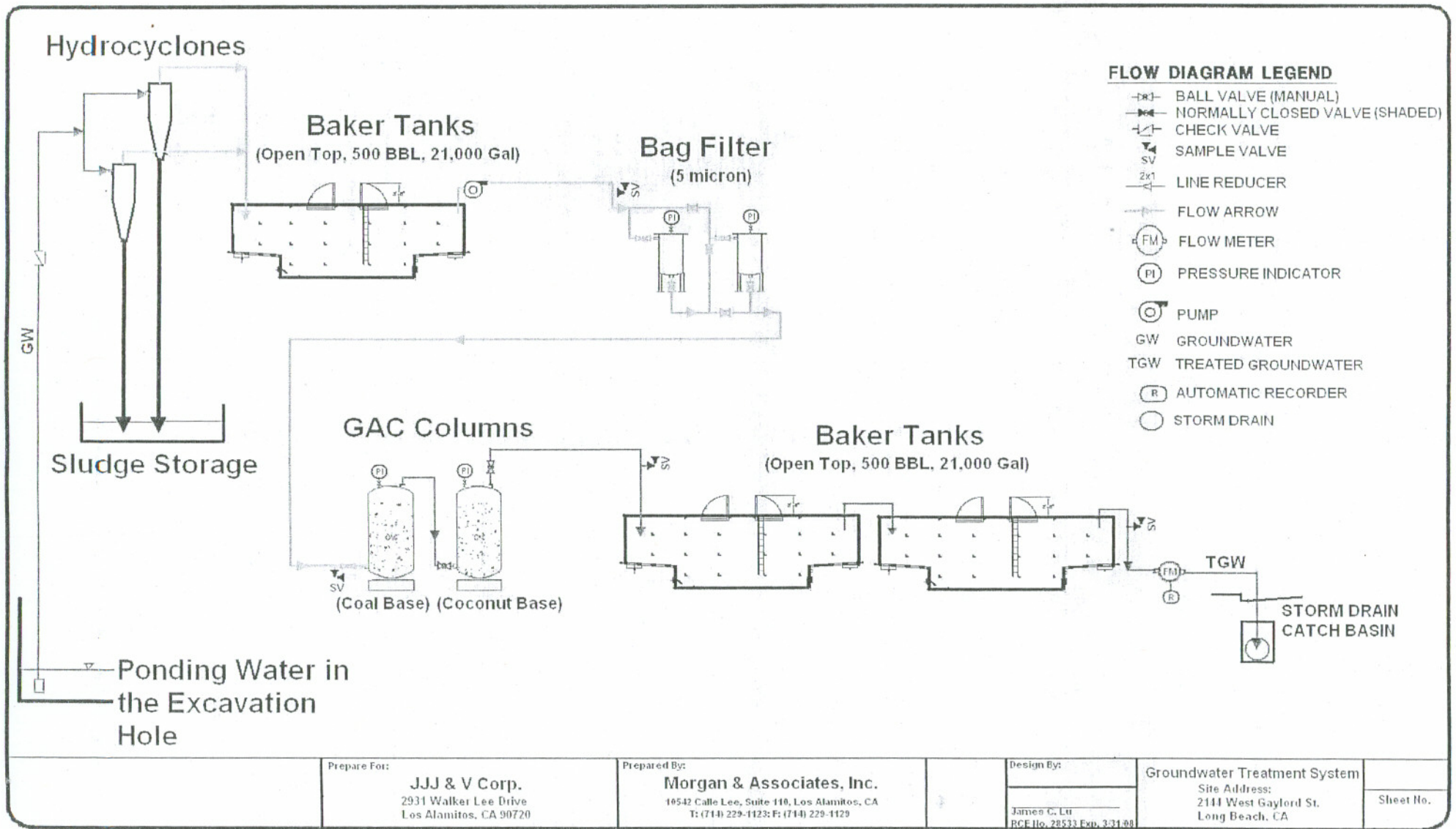
Figure 2. Treatment Process
