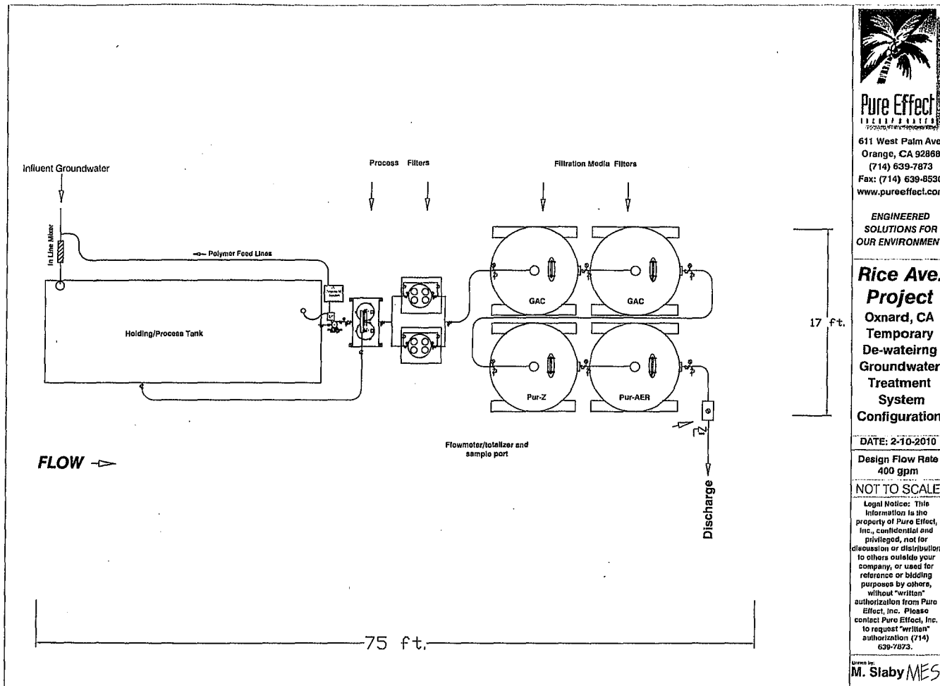
Figure 2-Treatment Schematic
