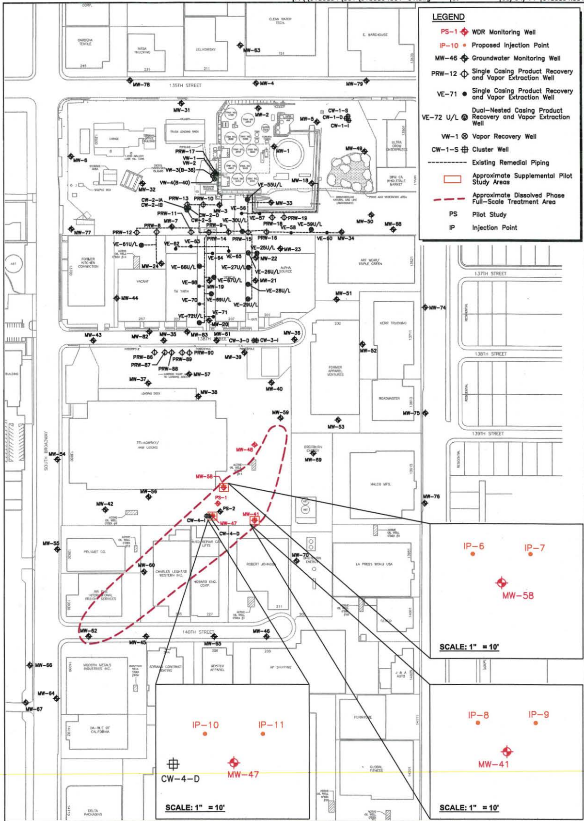
Figure 1 Proposed Supplemental Pilot Test ISCO Layout Phillips 66 Company Los Angeles East Terminal 0381 13500 South Broadway Los Angeles, California
