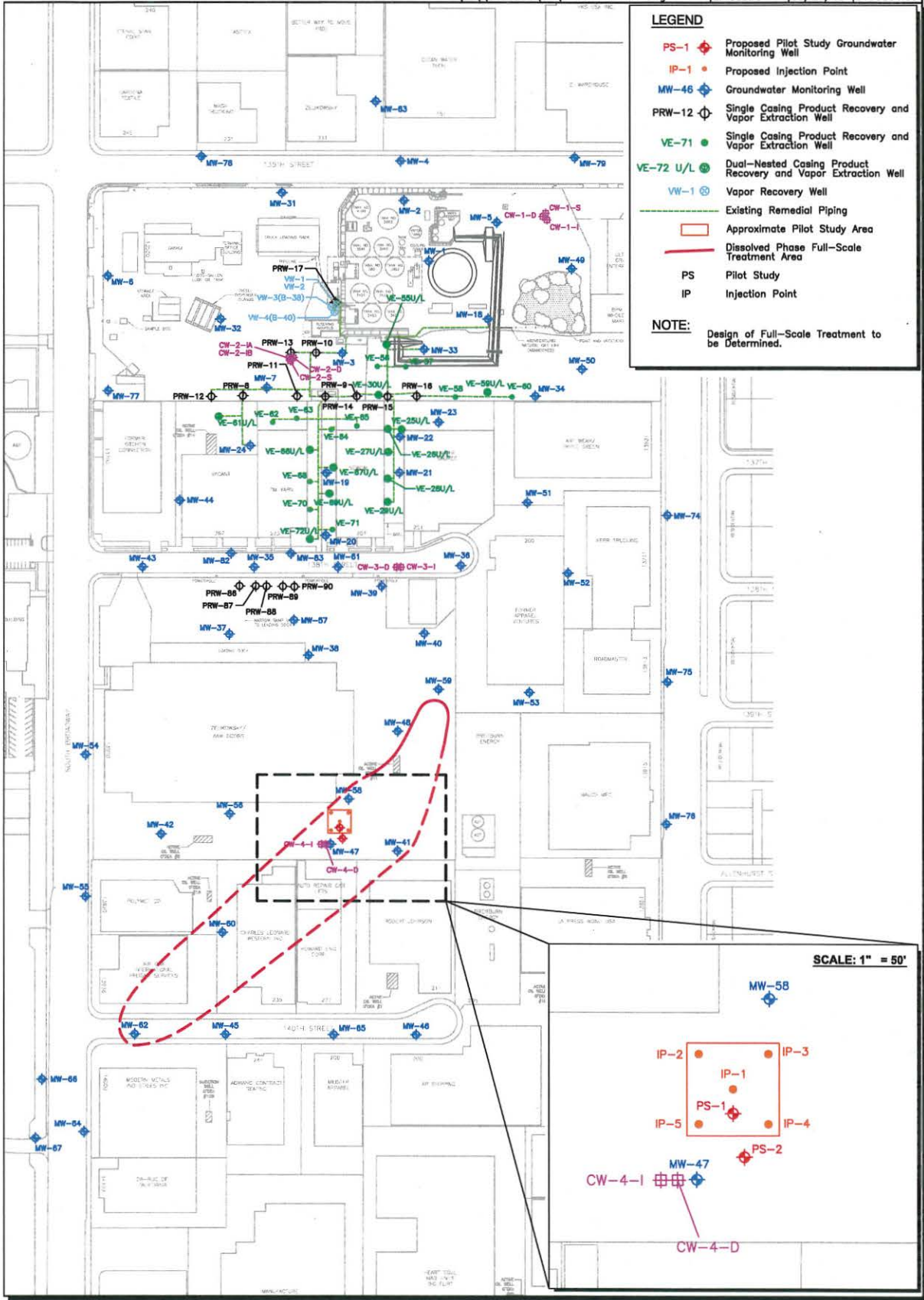
Figure 1 Pilot Test ISCO Layout Phillips 66 Company Los Angeles East Terminal 0381 13500 South Broadway Los Angeles, California ERM 03/13
