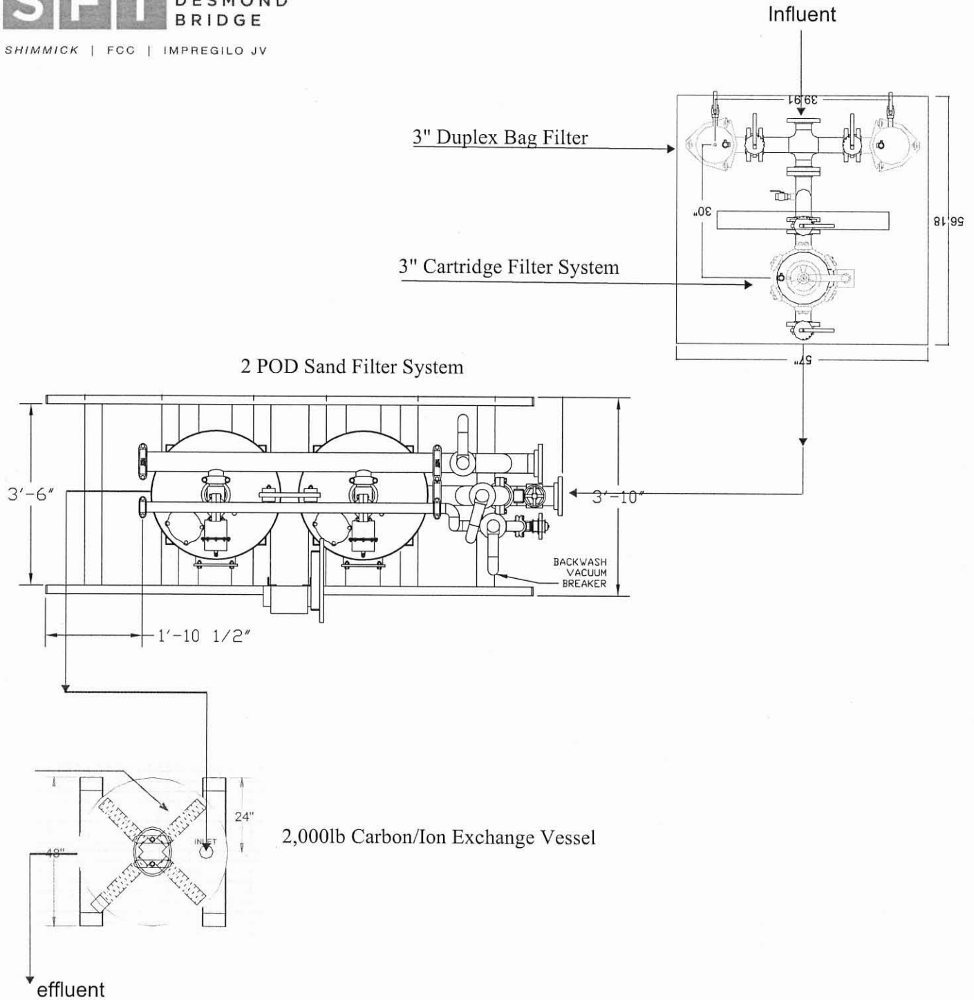
Figure 2. Treatment Process
