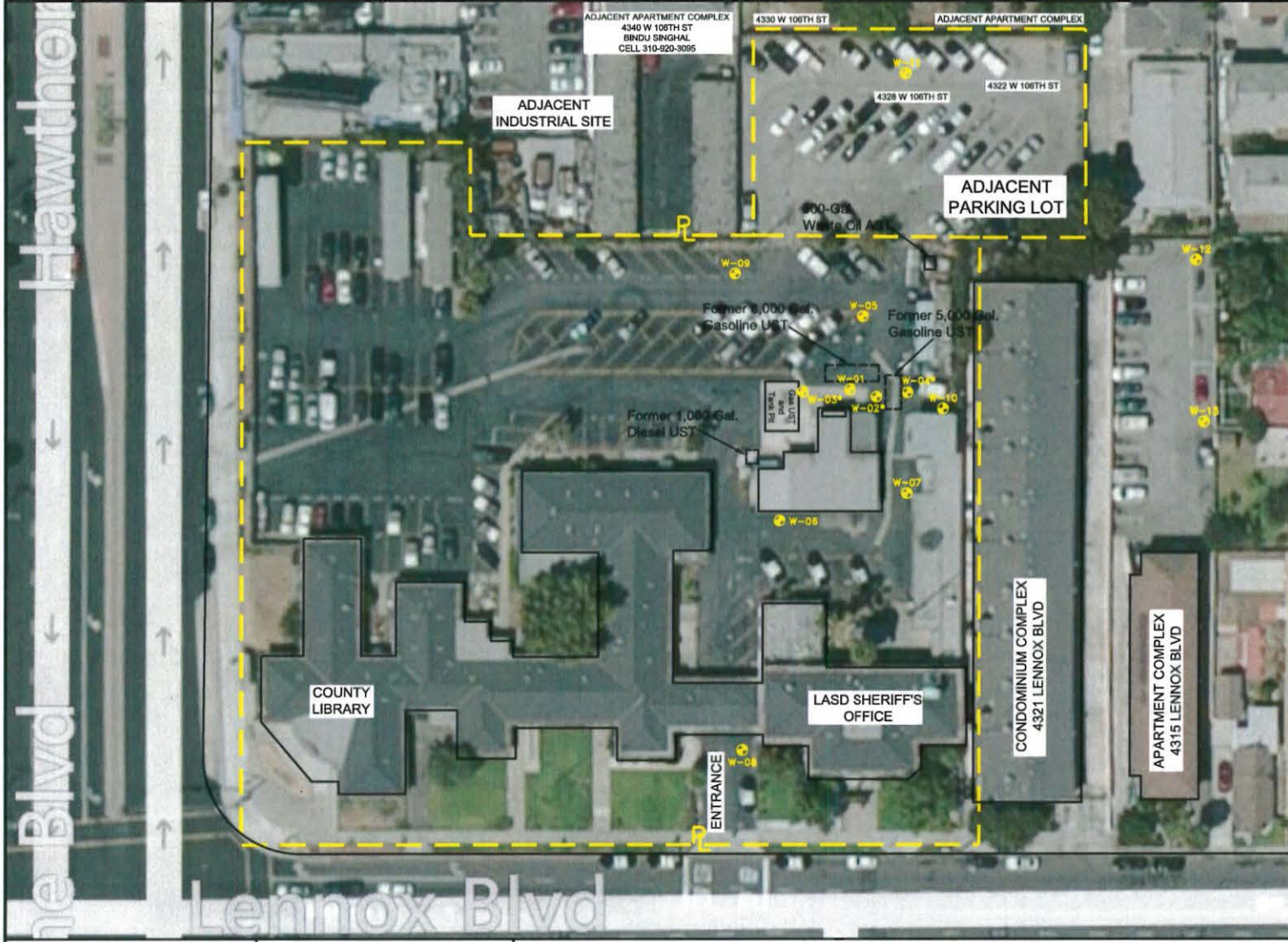
SITE PLAN LA COUNTY SHERIFF LENNOX STATION 4331 WEST LENNOX BOULEVARD, LENNOX, CALIFORNIA
