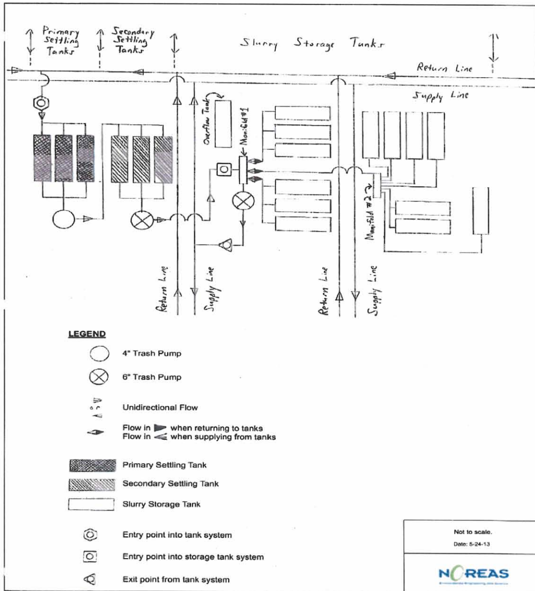
Figure 3. Wastewater Storage System
