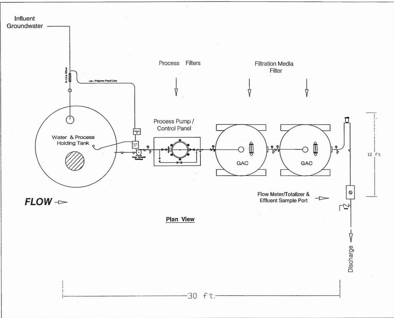
Figure 1. Schematic of treatment process
