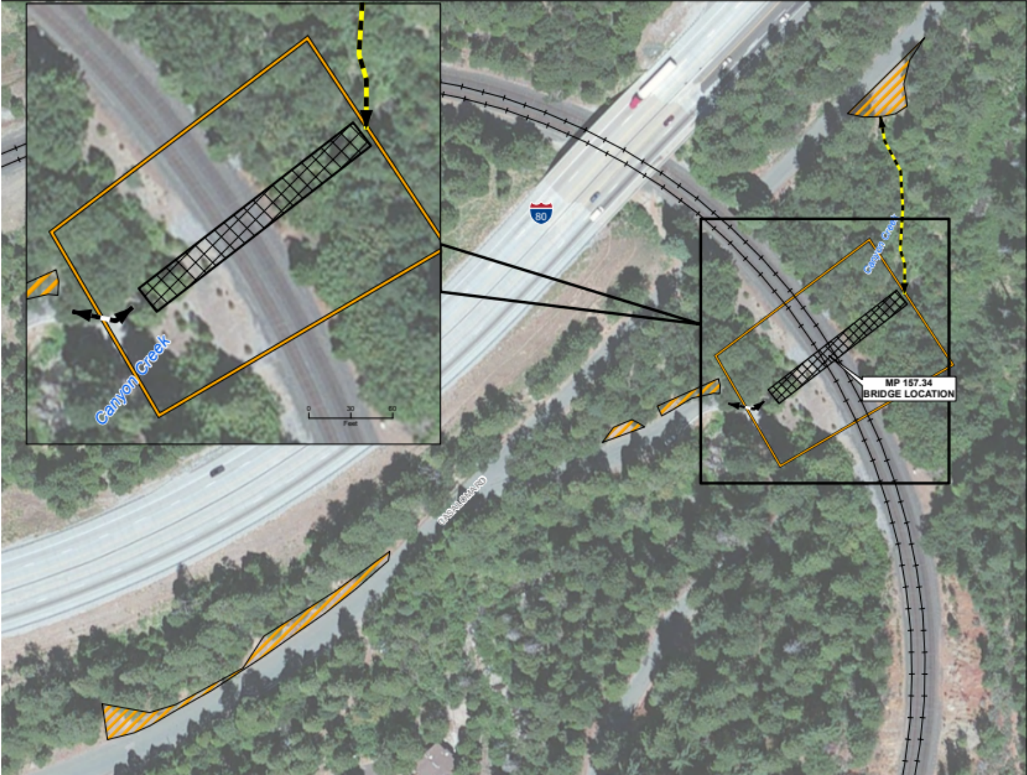
Figure 2: Culvert Map
