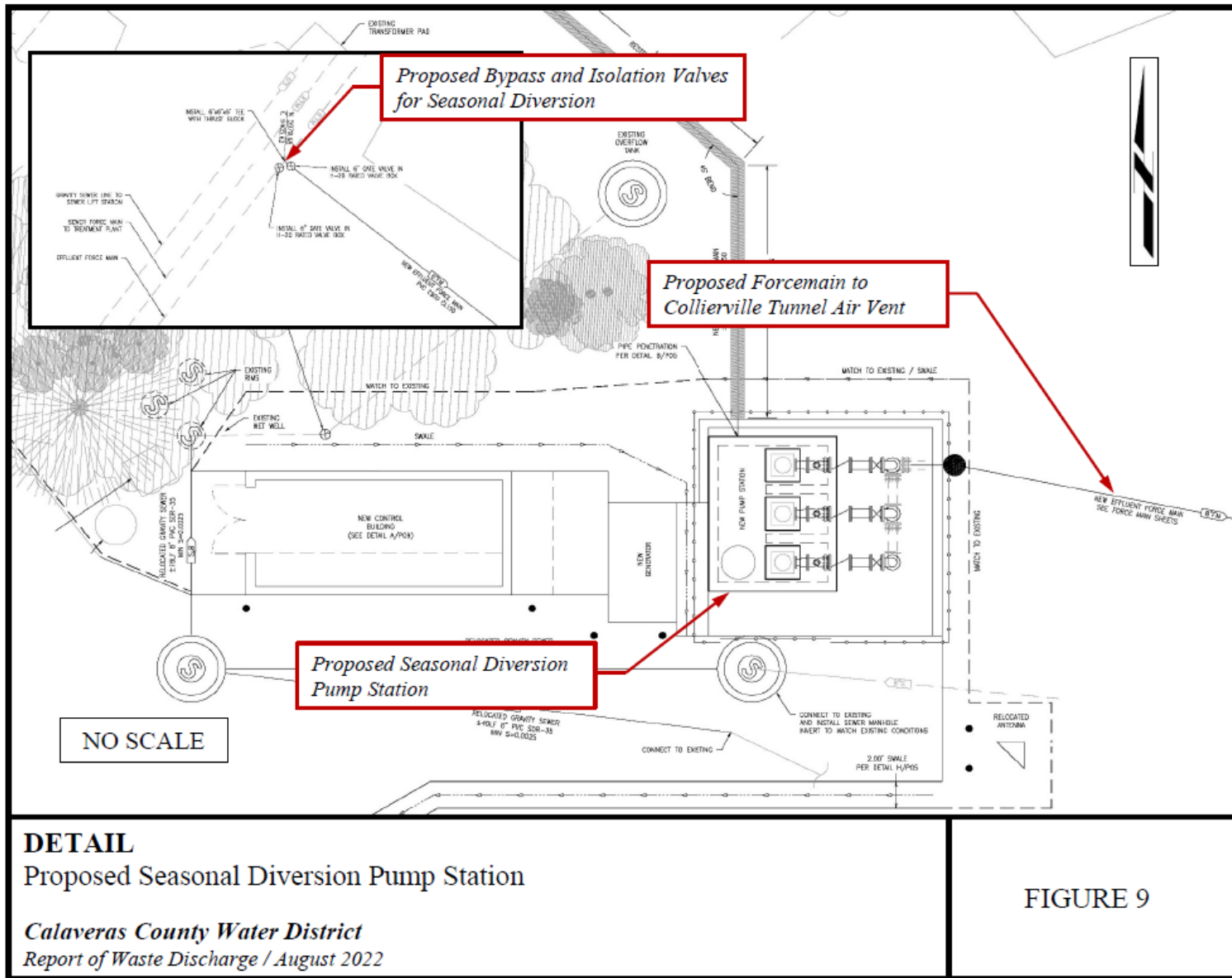
Figure C-3. Proposed Seasonal Diversion Pump Station Detail
