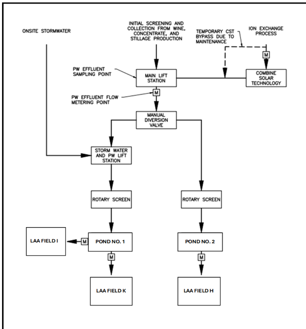
ATTACHMENT E – Process Flow Diagram
