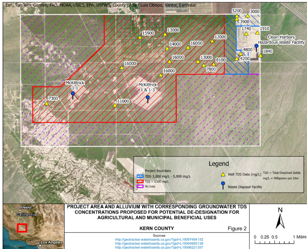
Figure 2. Project Area showing the whole area considered for de-designation (white box), the area where groundwater above the base of the CCE exceeds 5,000 mg/L TDS (red hashed area – Revised Project Area proposed for de-designation for both MUN and AGR beneficial uses), the area where groundwater above the base of the CCE is between 3,000 and 5,000 mg/L TDS (blue hashed area – Revised Project Area proposed for de-designation of only the MUN beneficial use), and the area where there is limited or no water quality data for groundwater above the base of the CCE (purple hashed area).
