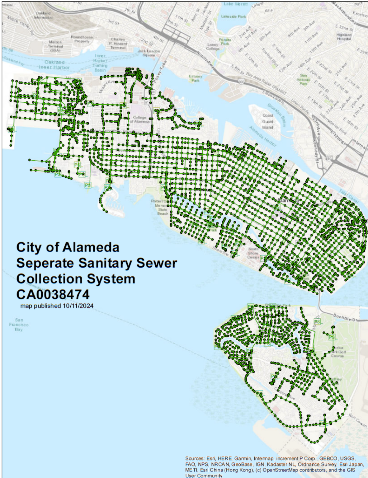
Figure B-1. Sewer Map
