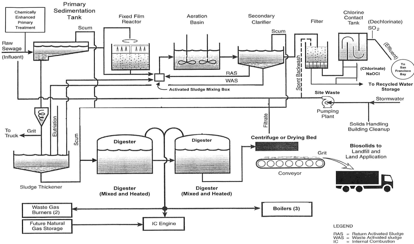
Plant Process Schematic
