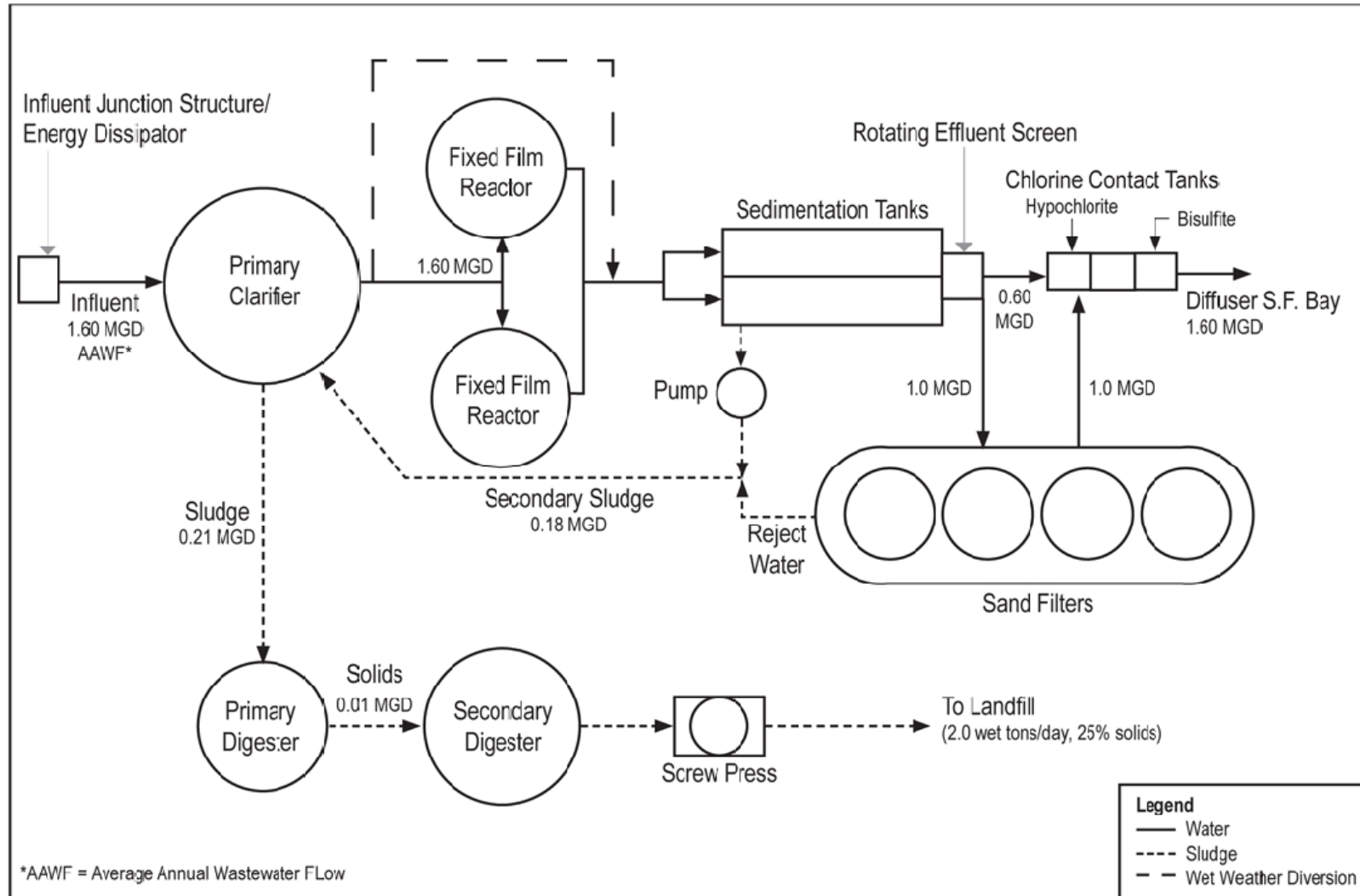
Figure C-1. Wastewater Treatment Plant Flow Schematic
