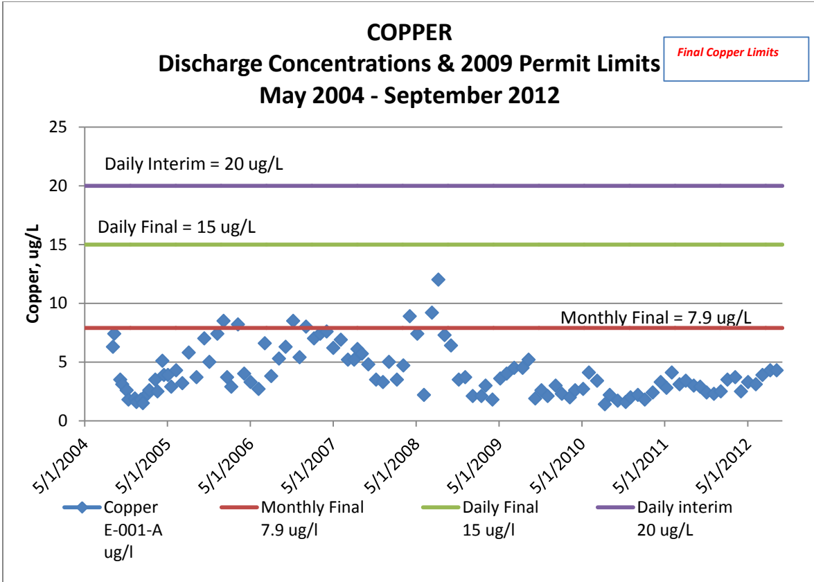
Figure 1. Copper Effluent Concentrations
