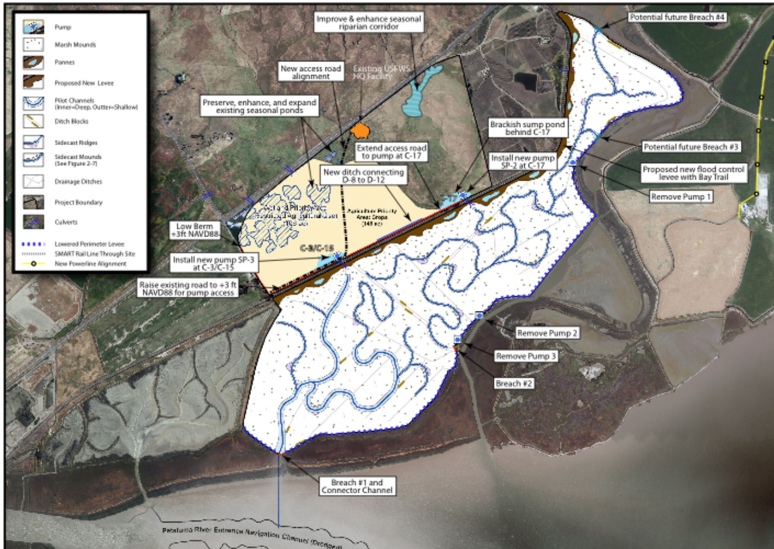
Figure 4. Sears Point Proposed Project
