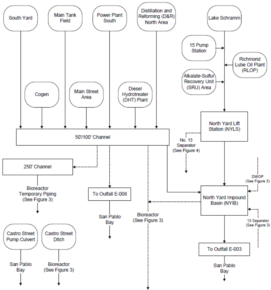
FIGURE 7 NPDES Richmond Refinery Process Area Rainwater System Flow Diagram 1
