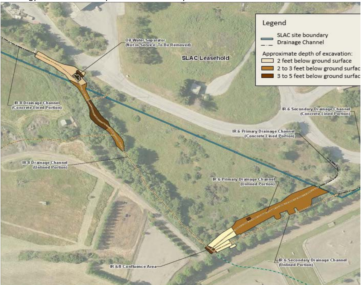
Figure 2. Project area showing planned excavation of IR-6 and IR-8 channels to remove PCB-contaminated sediment
