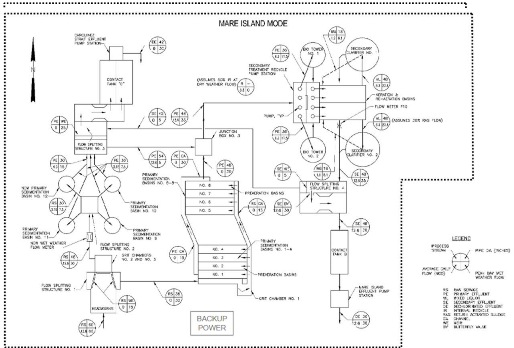
Attachment C – Process Flow: Figure 2. Wastewater Treatment Plant Process Flow Schematic, Mare Island Mode
