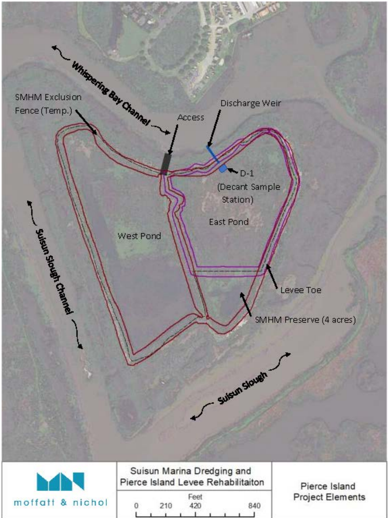
Figure 3. Site Plan
