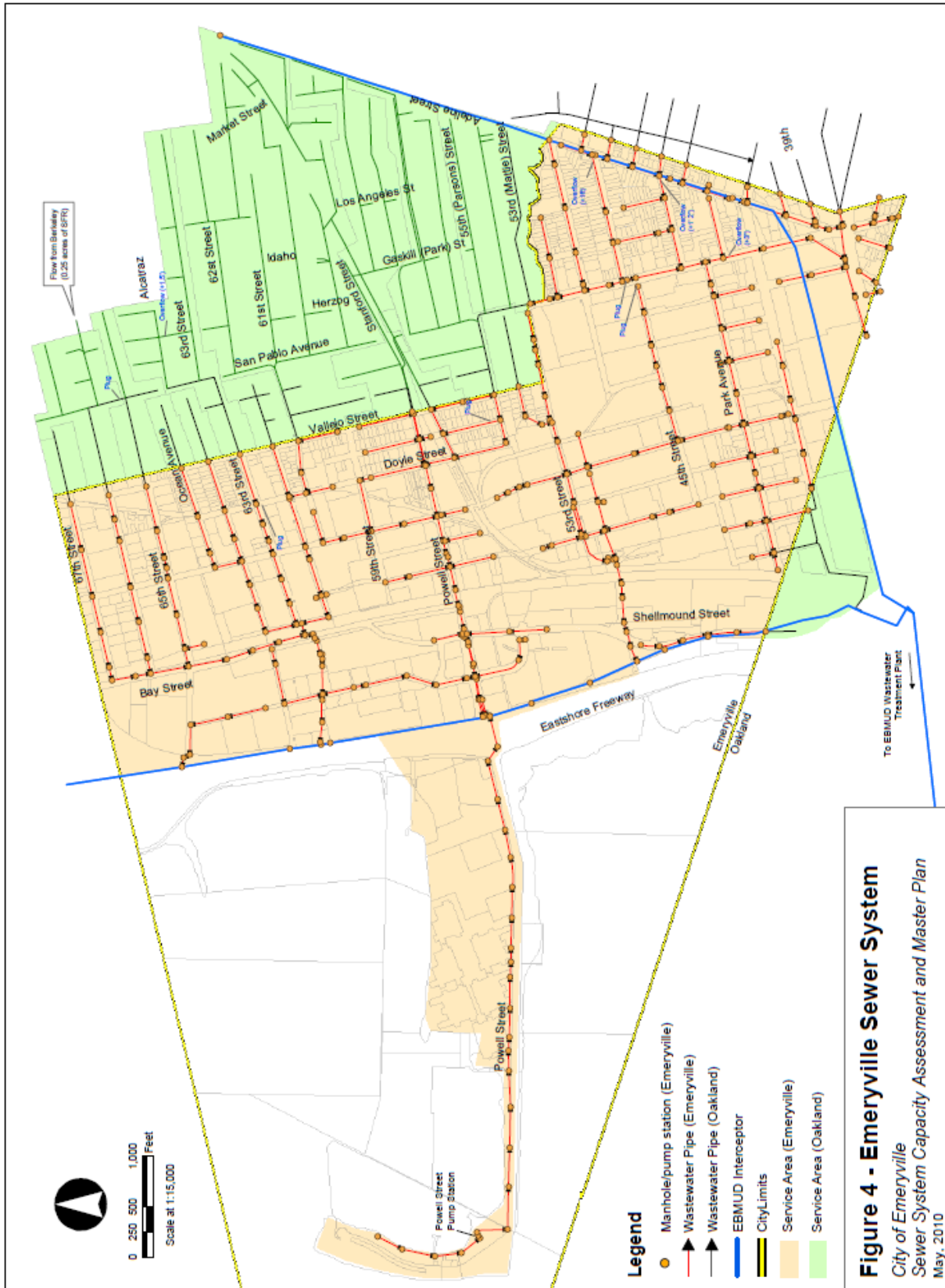
Figure B-1. Sewer Map
