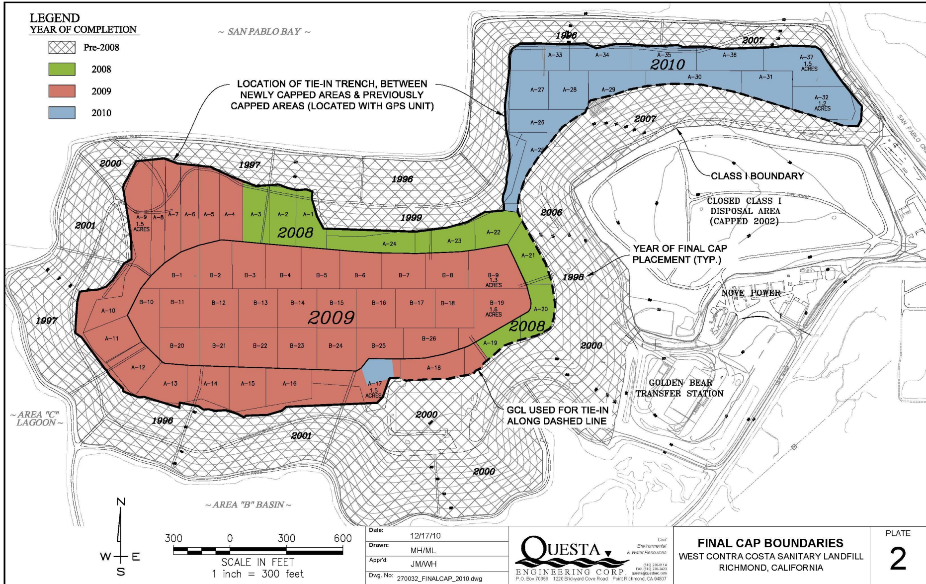
Figure 2. West Contra Costa Sanitary Landfill Closure Construction
