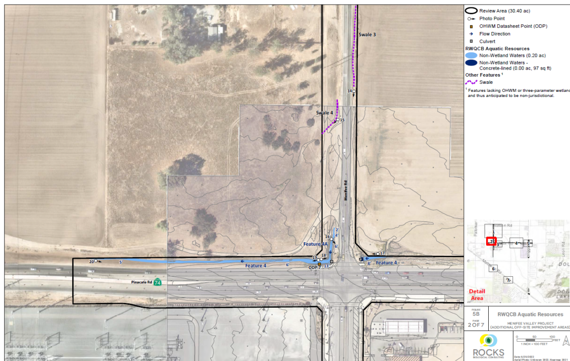
Figure 5. Impact to offsite drainage features (2)
