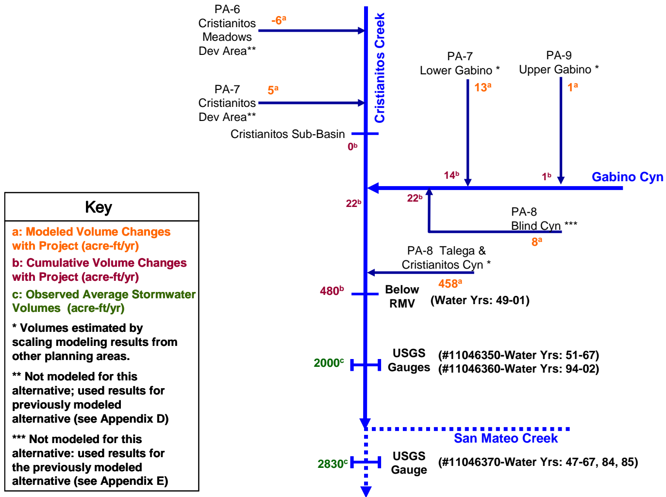
Figure7-3 Cumulative Increases in Annual Storm Runoff Volumes in the San Mateo Watershed
