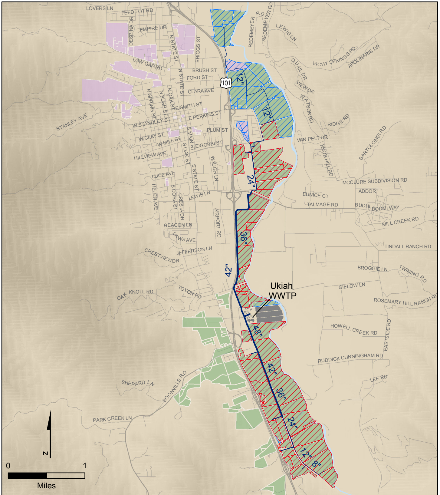
Figure 6.5 ALTERNATIVE 3B RECYCLED WATER MASTER PLAN CITY OF UKIAH
