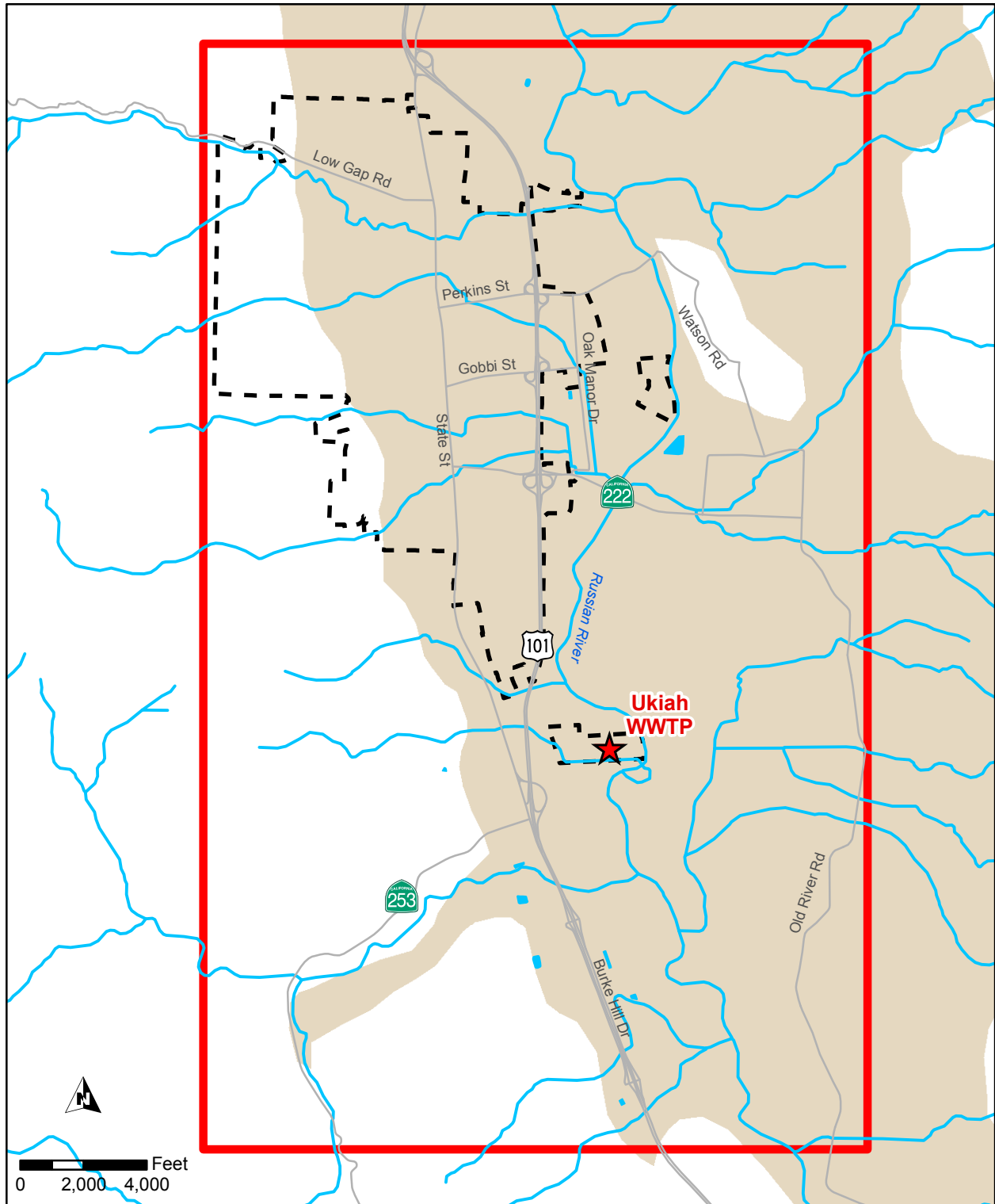
Figure 1.3 HYDROLOGIC FEATURES RECYCLED WATER MASTER PLAN CITY OF UKIAH
