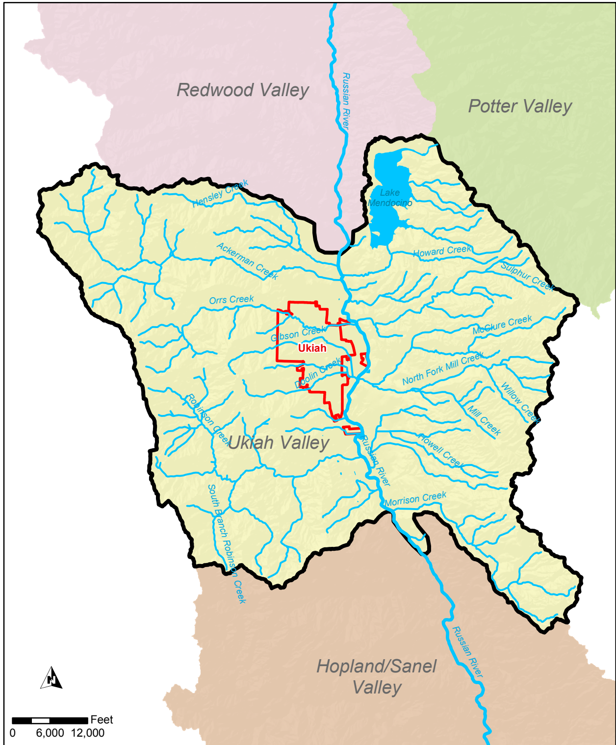
Figure 2.1 UKIAH VALLEY AND NEIGHBORING WATERSHEDS RECYCLED WATER MASTER PLAN CITY OF UKIAH
