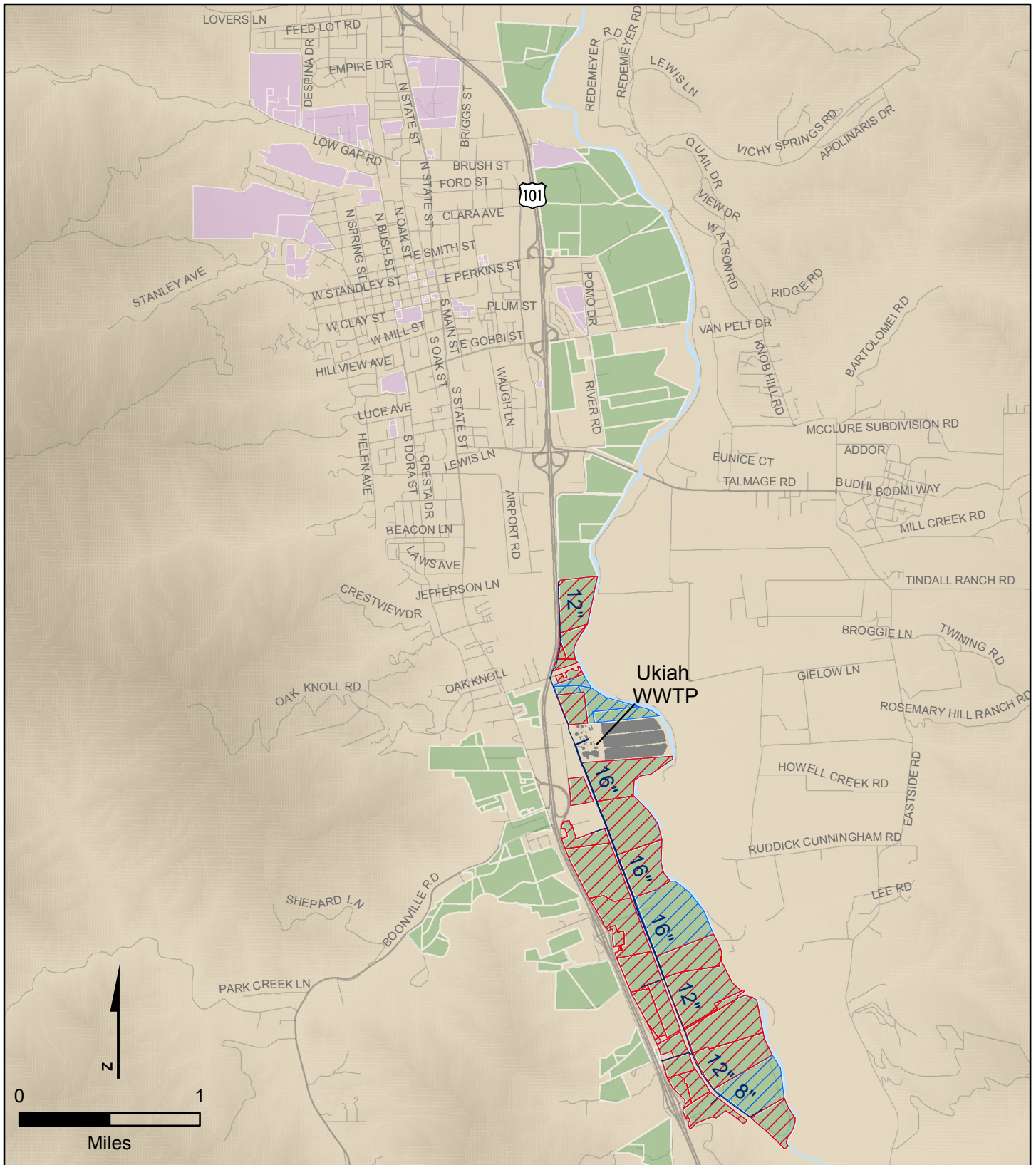
Figure 6.3 ALTERNATIVE 2 RECYCLED WATER MASTER PLAN CITY OF UKIAH
