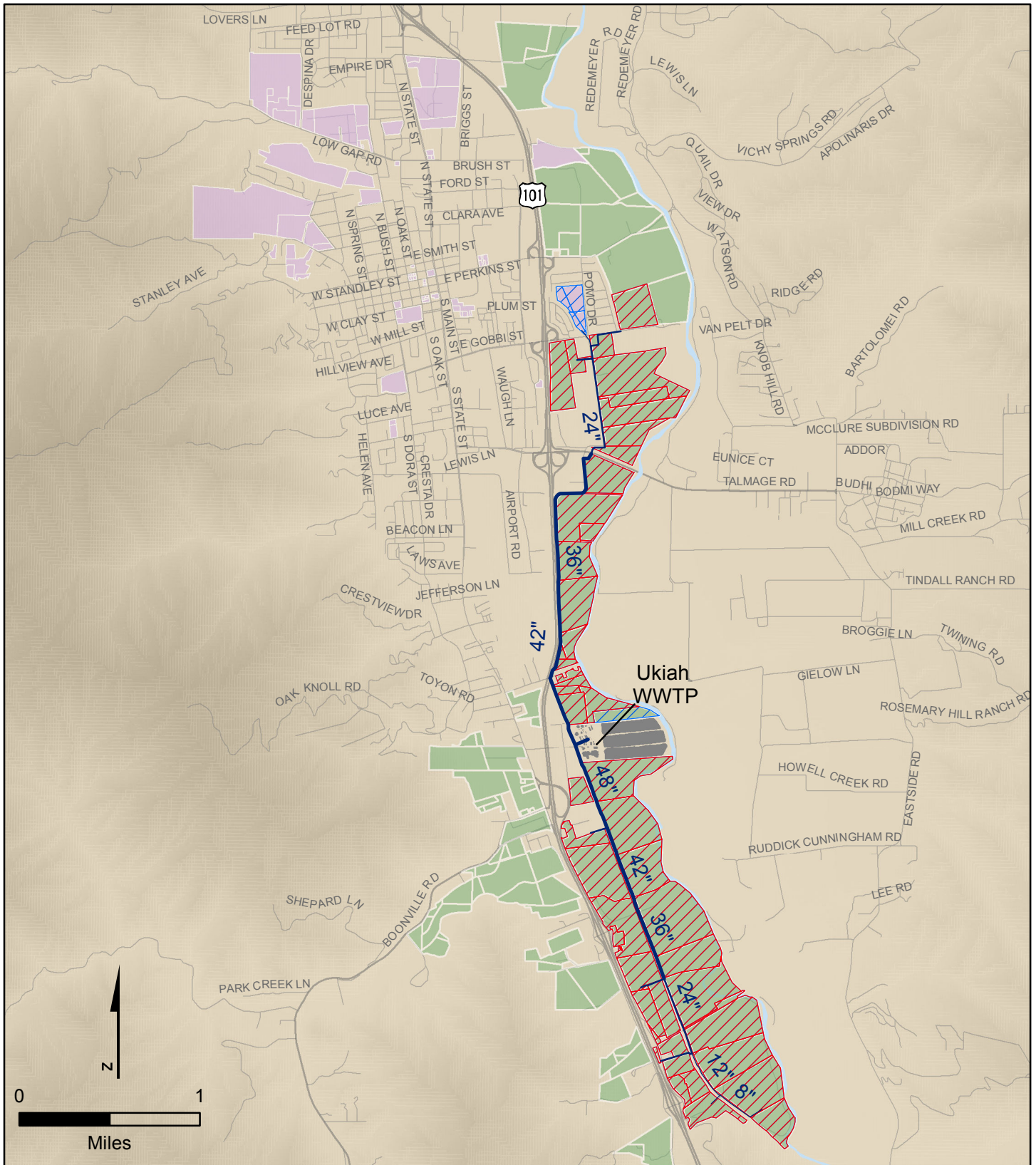
Figure 6.4 ALTERNATIVE 3 RECYCLED WATER MASTER PLAN CITY OF UKIAH
