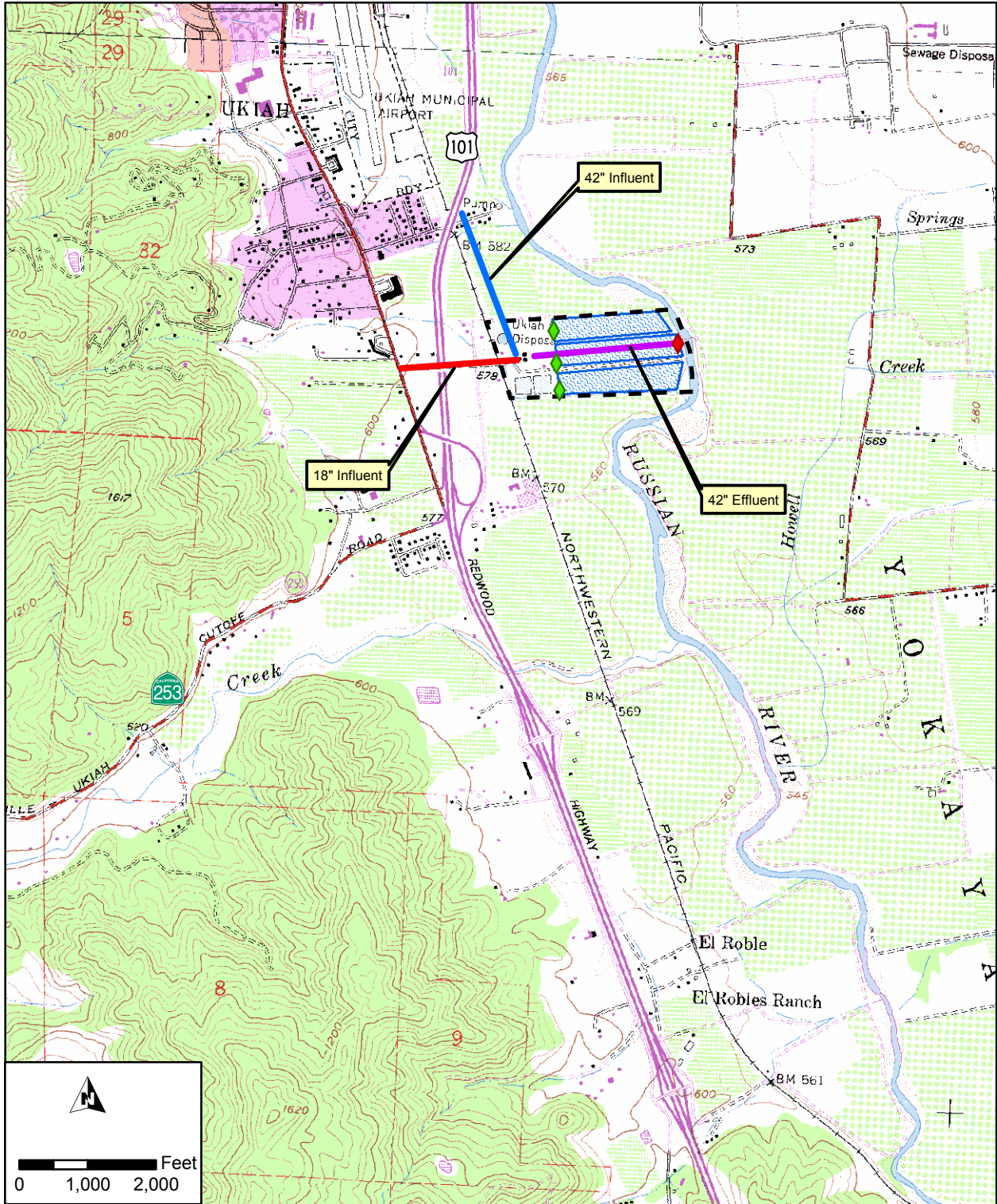
Figure 3.2 UKIAH WWTP OVERVIEW RECYCLED WATER MASTER PLAN CITY OF UKIAH
