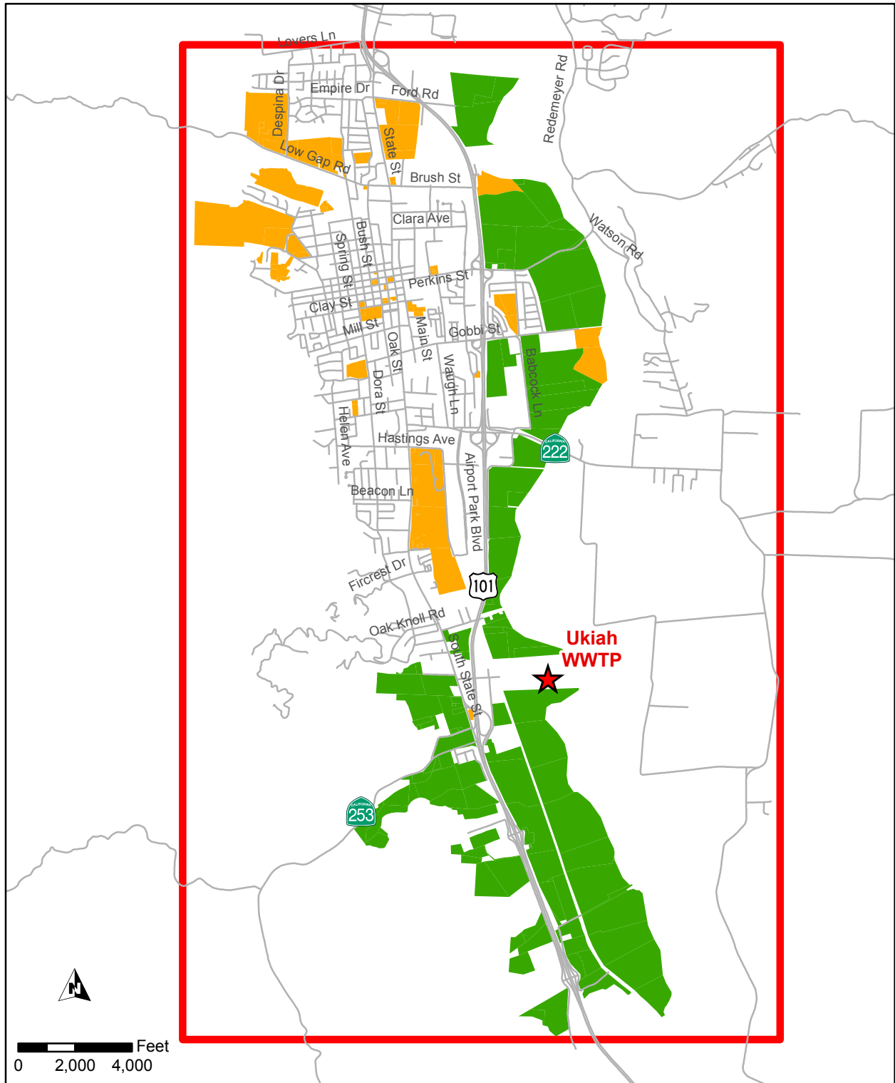
Figure 5.1 POTENTIAL RECYCLED WATER USE SITES RECYCLED WATER MASTER PLAN CITY OF UKIAH
