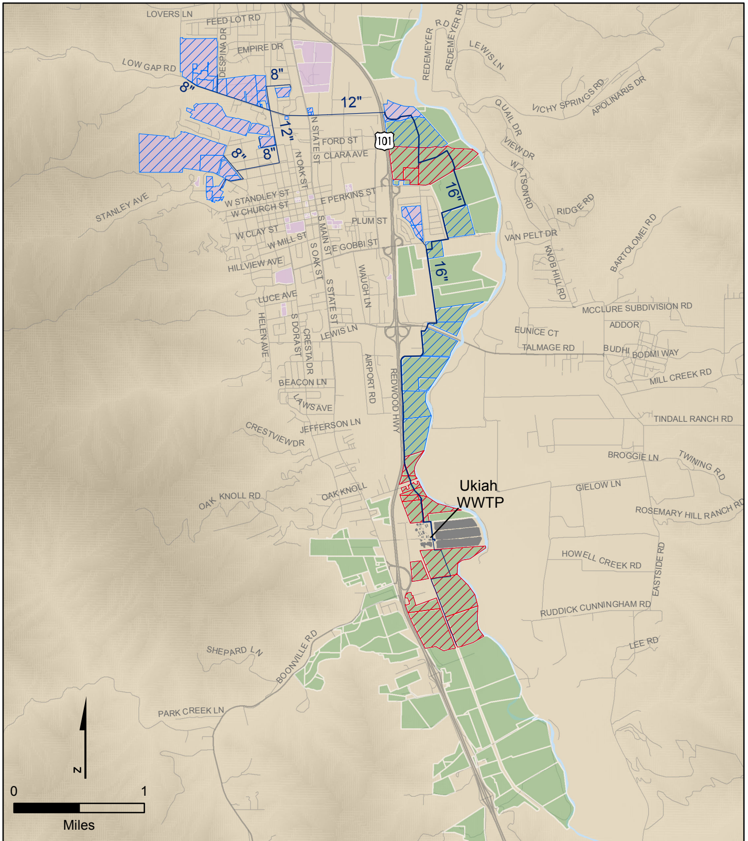
Figure 6.6 ALTERNATIVE 4 RECYCLED WATER MASTER PLAN CITY OF UKIAH
