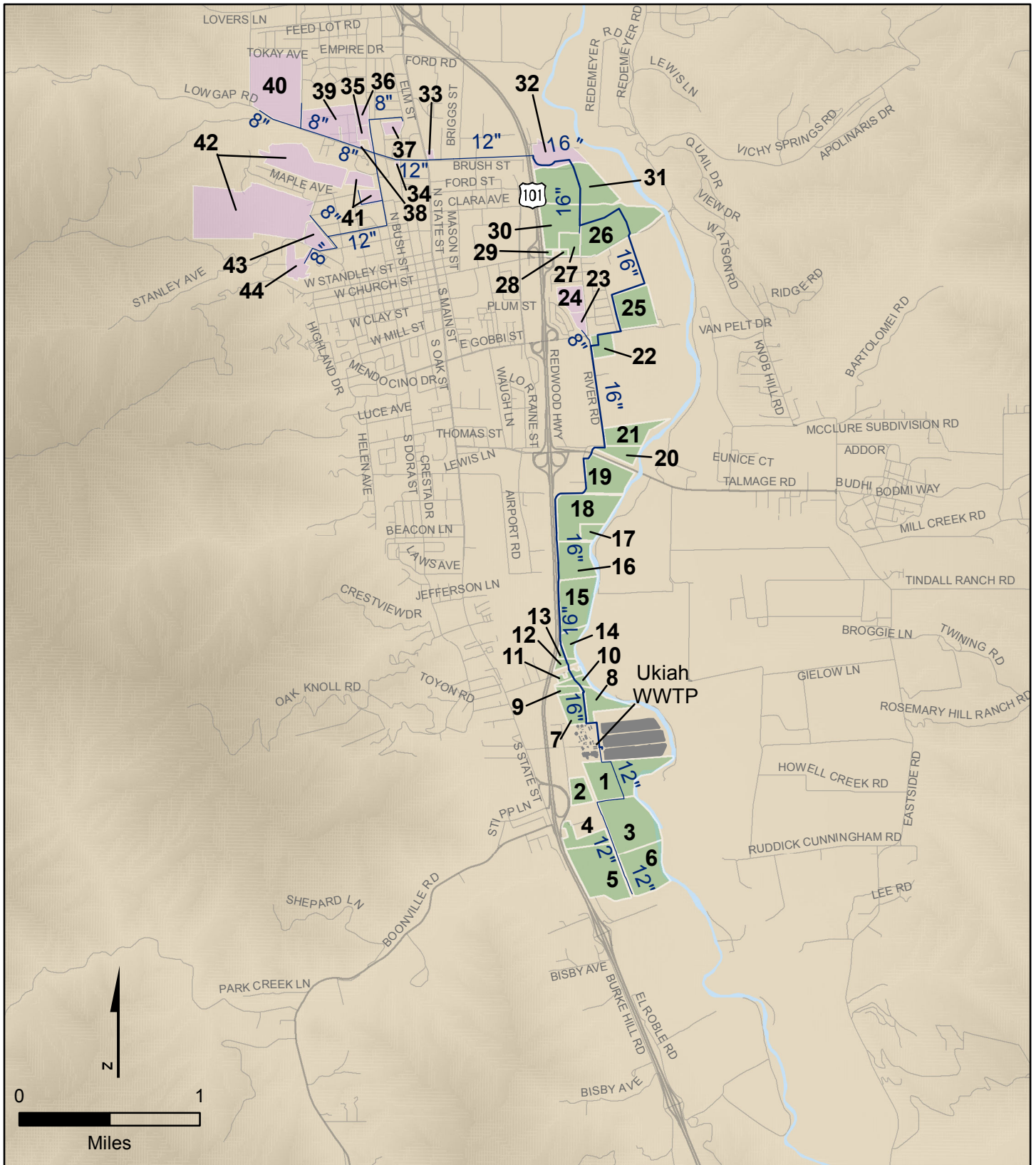
Figure 7.1 RECOMMENDED ALTERNATIVE RECYCLED WATER MASTER PLAN CITY OF UKIAH
