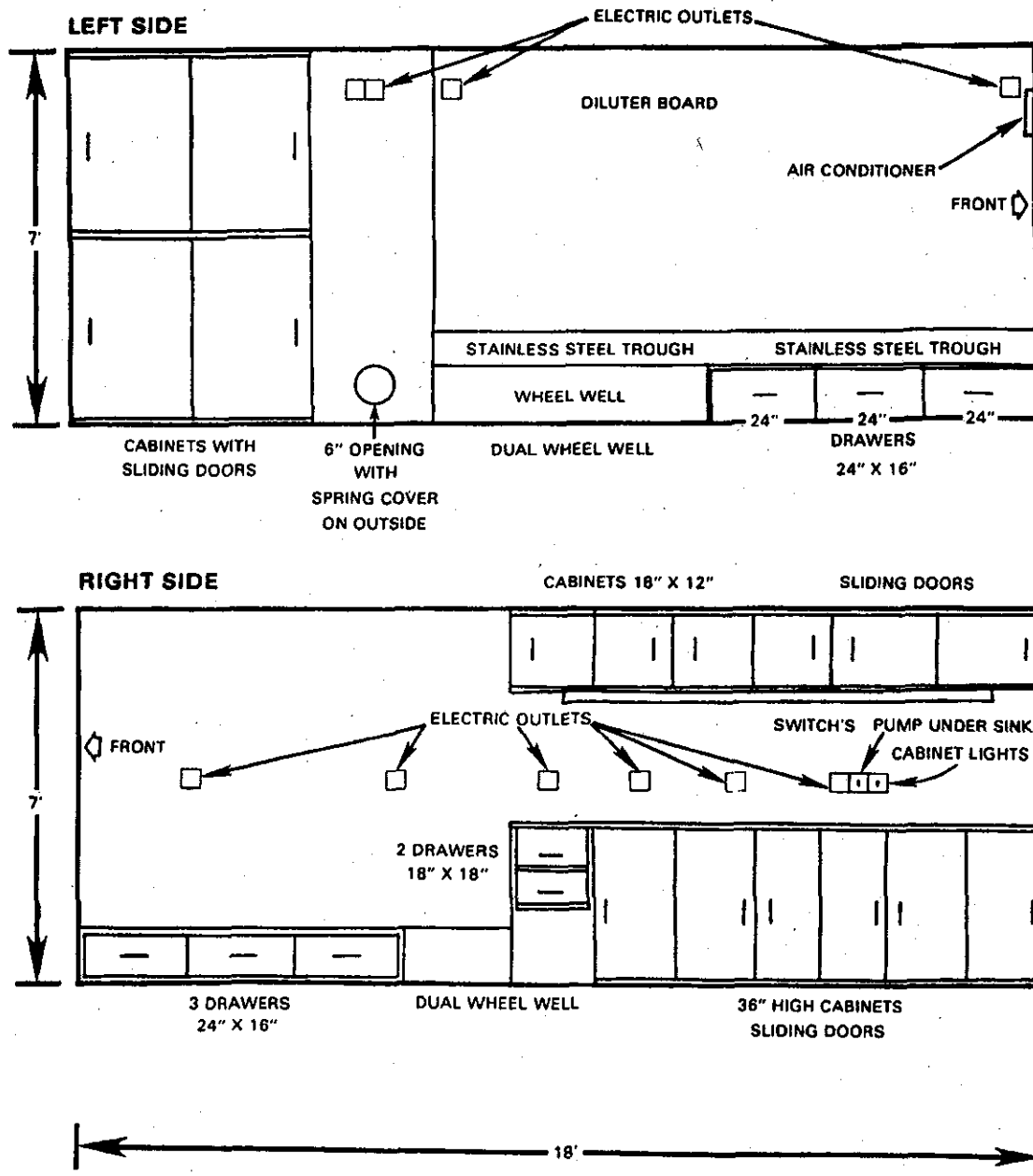
Figure 3. Mobile bioassay laboratory, tandem-axle trailer, internal views of side walls.
