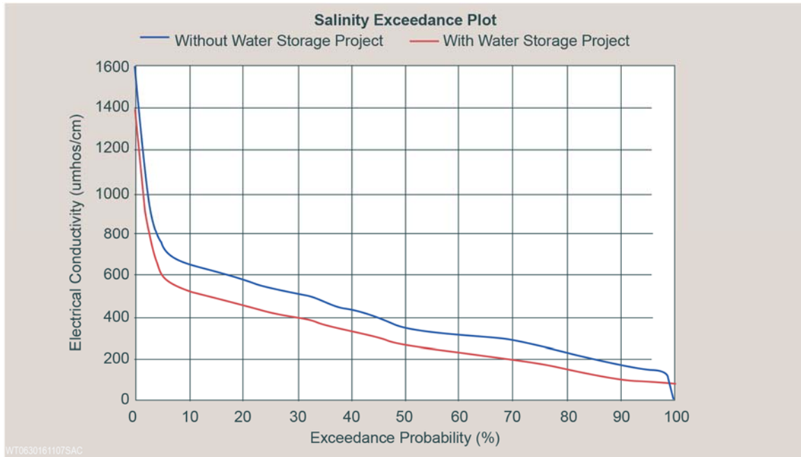
Figure 4-8-8. Example Exceedance Plot.
