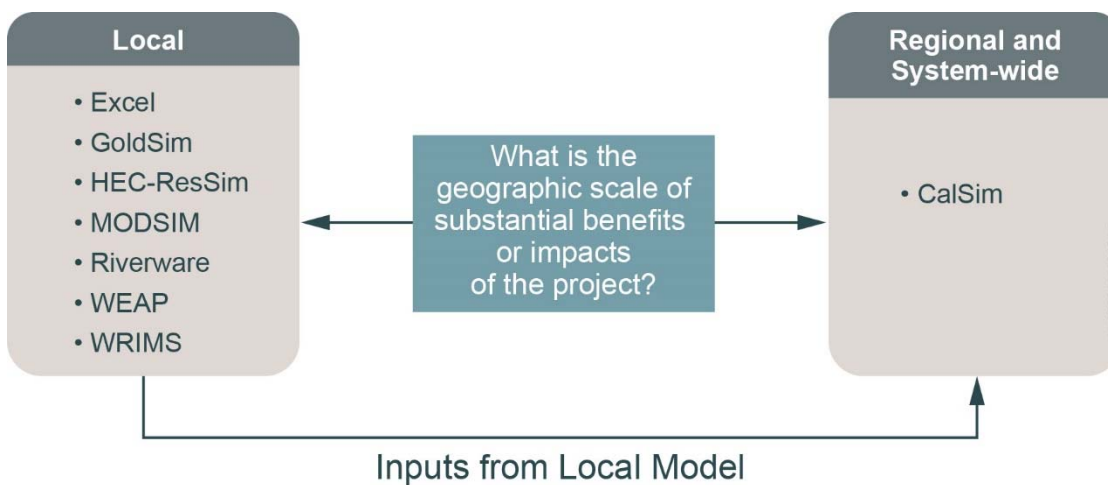
Figure 4-54-5. Flow Chart for Determining Appropriate Approach.
