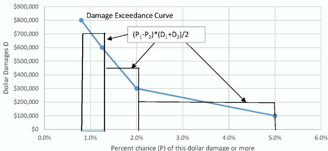
Figure 5-35-3. EAD and the Damage Exceedance Curve.
