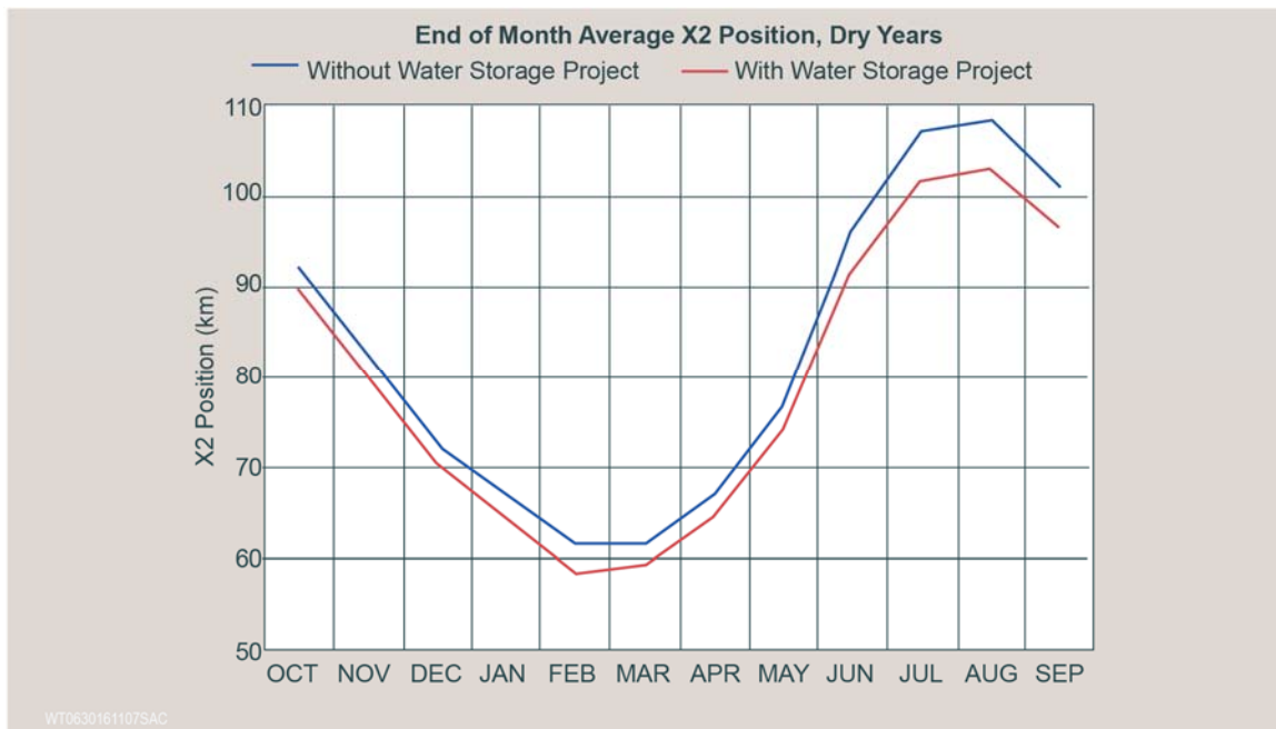
Figure 4-7-7. Example X2 Position Plot.
