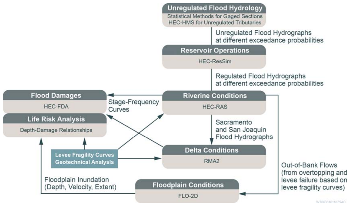
Figure 4-114-11. Schematic of CVFPP Process and Tools for Calculating Flood Damages.
